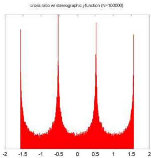
Fig. 2. Probability density function of stereographic permutation invariants
