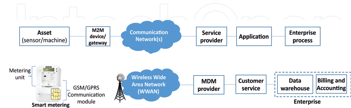
Figure 5. Generic M2M system (top) and corresponding system in smart metering (bottom).
