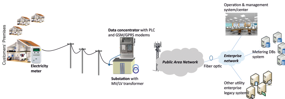
Figure 8. Reference architecture smart metering using PLC.
