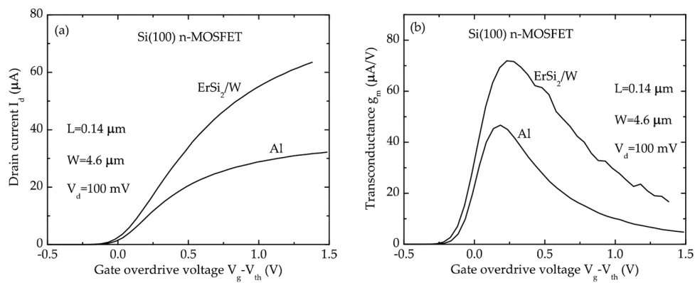
Figure 4. (a) Drain current and (b) transconductance versus gate overdrive voltage for n-MOSFETs featuring Al and \text{ErSi}_2/\text{W} contacts. Copyright 2011 The Japan Society of Applied Physics [8].
