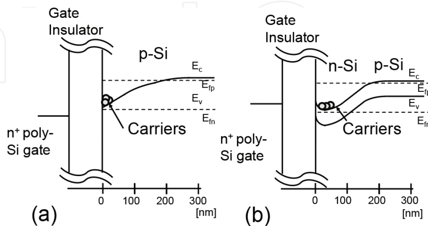
Figure 11. Diagrams of surface channel (a) and buried-channel MOSFETs. The bias condition was set at V_{BS} = 1.5 V and I_{DS} = 100 nA.
