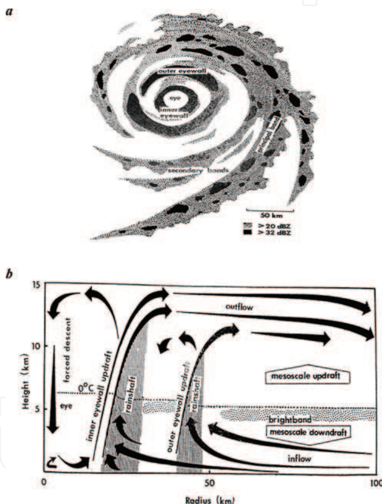
Figure 5. Two schematics of TC structures from [109]. (a) Horizontal cross-section of structural features as presented by radar. (b) Vertical cross-section of the same structural features and their relation to the secondary circulation described in Eliassen [110] and Shapiro and Willoughby [111] (adapted from Willoughby (1995)).
