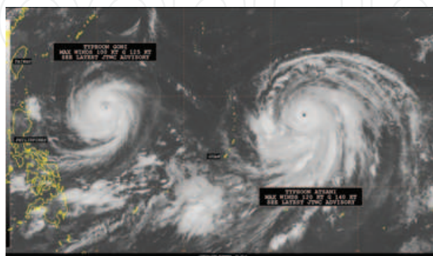
Figure 3. Japanese satellite Himawari-8 IR image of Typhoons Goni and Atsani at 1800 UTC Aug 18, 2015 (adapted from the Joint Typhoon Warning Center (JTWC) at http://www.usno.navy.mil/JTWC ).
