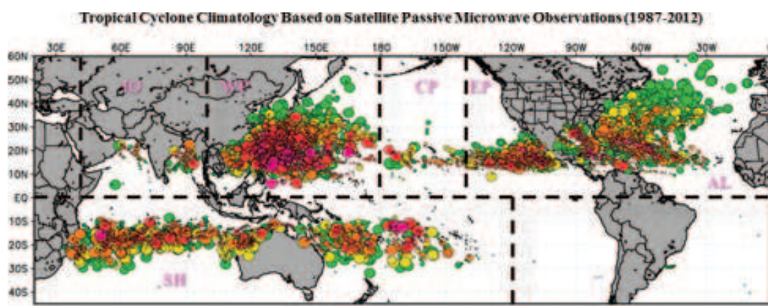
Figure 1. Tropical cyclone (TC) climatology from satellite passive microwave sensor measurements during 1987–2012. The sizes of the circles are proportional to their eye radius, while the colors show TC's intensity with warmer color for more intense TC. AL, CP, EP, IO, SH, and WP defined by Joint Typhoon Warning Center (JTWC) are used for storm basins of North Atlantic, Central North Pacific, Eastern North Pacific, Northern Indian Ocean, Southern Hemisphere and Western North Pacific, respectively.
