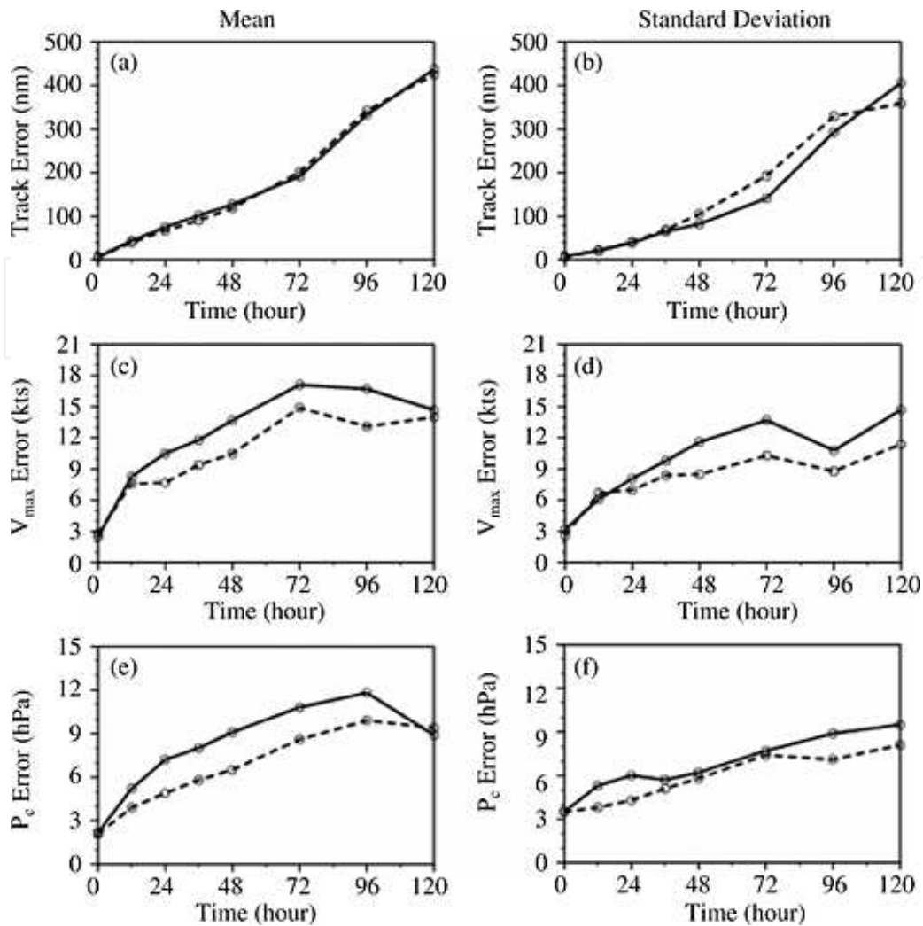
Figure 13. Mean forecast errors and standard deviations as functions of forecast lead time for TC track (a and b), maximum wind V_{\max} (c and d), and minimum center pressure P_c (e and f) of CTRL2 (solid) and CTRL2+ATMS (dashed) of the four landfall storms (adapted from Zou et al. (2013). Reproduced by permission of American Geophysical Union).
