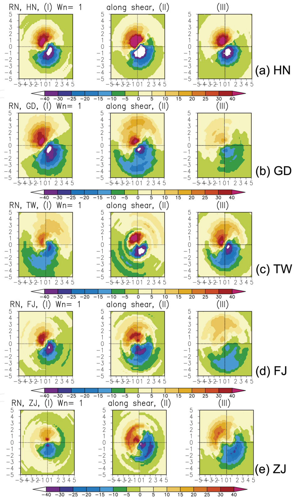
Figure 10. The wavenumber 1 rainfall asymmetry (mm) relative to the storm vertical wind shear. The shear vector is aligned with the positive y axis (upward). The x and y axes are distance (°) from the TC center (origins). Stage (I) is 24 hr prior to, stage (II) is at the time of, and stage (III) is 24 hr after landfall. The color scale indicates the amplitude of the asymmetry relative to the storm motion (adapted from Yu et al. (2014)). ©American Meteorological Society. Used with permission).
