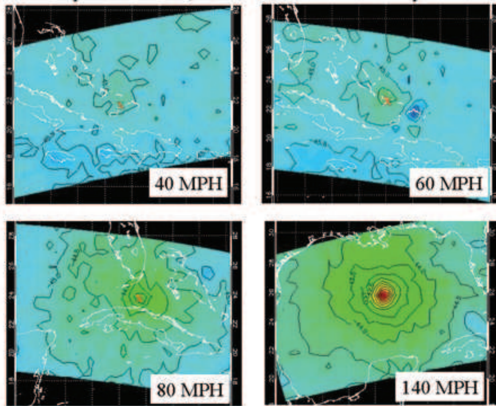
AMSU Temperatures at 40,000 ft for Hurricane Rita September 18-21
