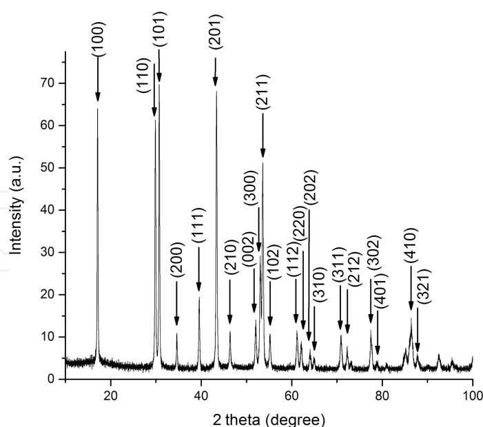
Figure 8. XRD spectrum of the upconversion phosphor powder baked for 1 h at 400°C with the diffraction peaks attributed to the hexagonal \beta -phase of \text{NaYF}_4 .
