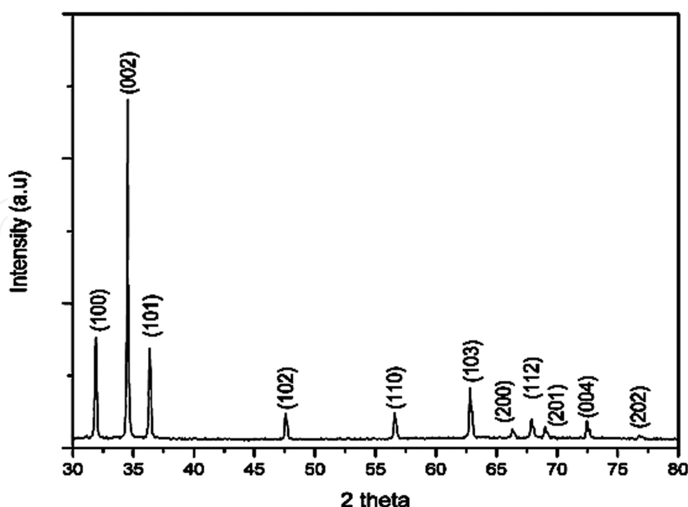
Figure 9. XRD spectrum of the prepared AZO PLD target with the diffraction peaks attributed to ZnO.
