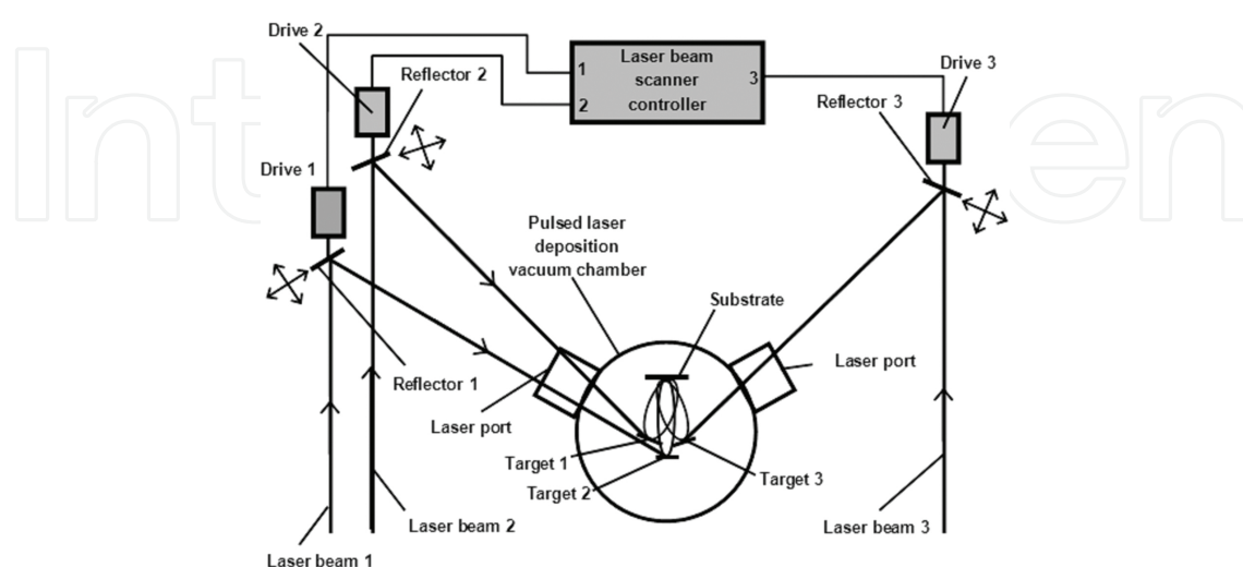
Figure 1. The schematic of the MBMT-MAPLE/PLD system [60].
