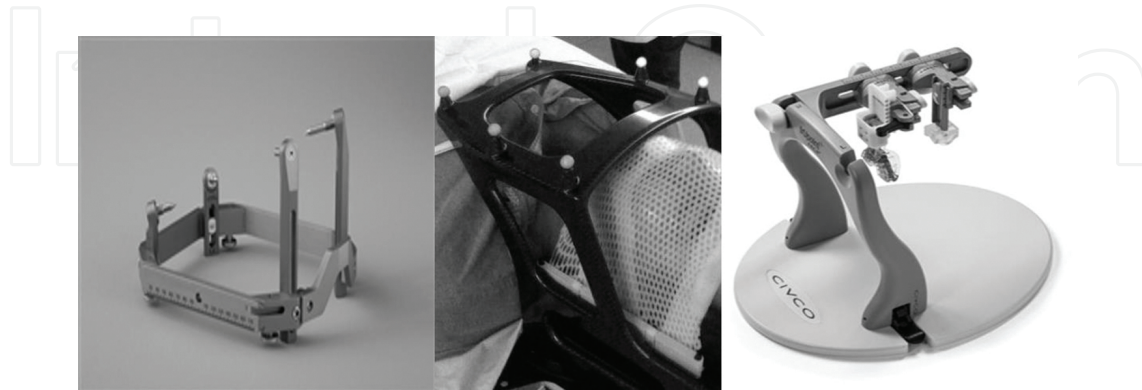
Figure 10. Left: Leksell frame; middle: Brainlab localization array mask; and right: CIVCO mask.
