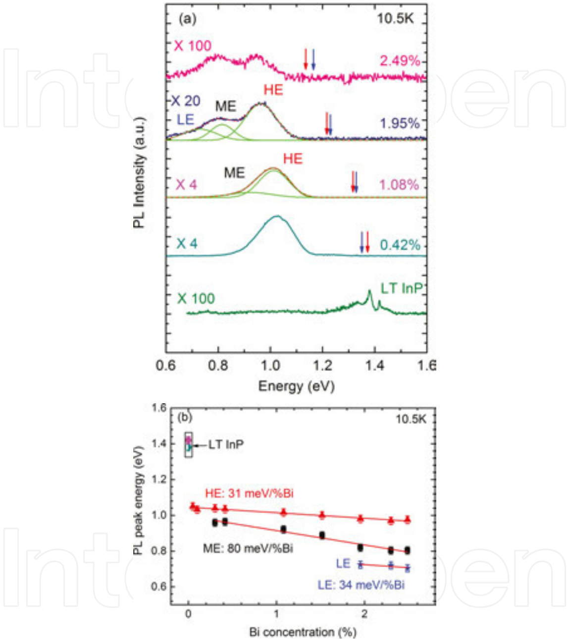
Figure 14. (a) PL spectra of InP 1-x Bi x samples with various Bi concentrations and LT InP reference sample at 10.5 K. Red arrows point to the theoretical band gap values of InP 1-x Bi x following the 106 meV/% Bi. Blue arrows point to the band gap measured from absorption spectra following the 91 meV/% Bi. The green curves are the Gaussian peak fitting. The red solid curve is the sum of the fitted lines. (b) PL peak energy evolution versus Bi concentration. The red solid line is a linear fit of HE (slope = 31 meV/% Bi); the black solid line is a linear fit of ME (slope = 80 meV/% Bi); the blue solid line is a linear fit of LE (slope = 34 meV/% Bi).
