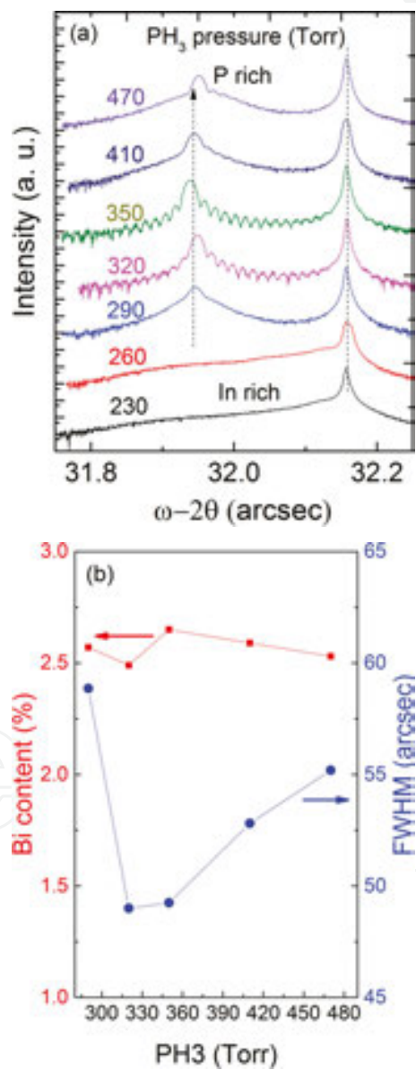
Figure 5. (a) HRXRD (004) \omega/2\theta rocking curves of InP 1-x Bi x layers grown at varying PH 3 pressures; (b) dependence of the Bi content and the FWHM on the PH 3 pressure.
