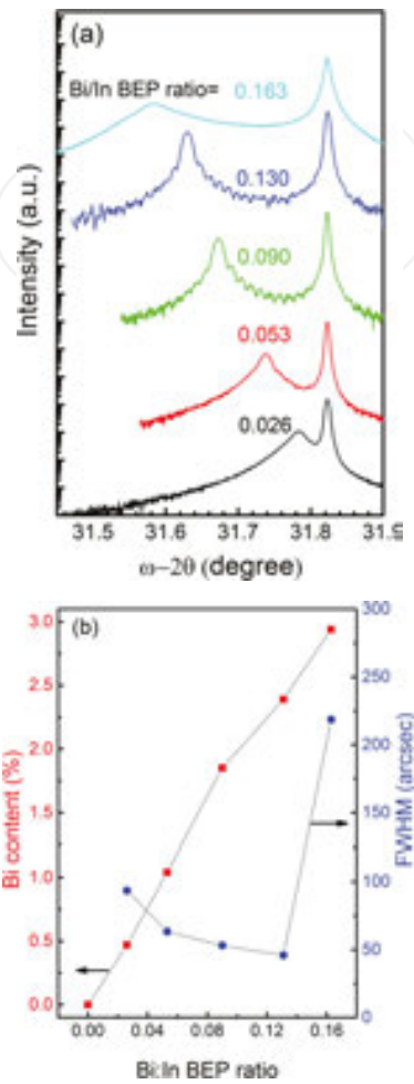
Figure 3. (a) HRXRD (004) \omega/2\theta rocking curves from \text{InP}_{1-x}\text{Bi}_x samples grown at varying Bi flux; (b) dependence of the Bi content and the FWHM on Bi/In BEP ratio.
