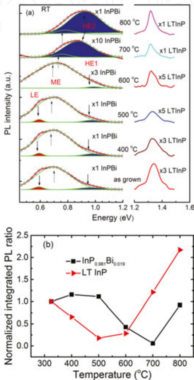
Figure 17. (a) PL spectra of \text{InP}_{1-x}\text{Bi}_x ( x = 0.019 ) and LT grown InP as reference at room temperature. The dotted lines are measured data. The green and red lines are the Gaussian peak fitting and the sum of fitted lines, respectively. (b) The normalized integrated PL intensity in respect of the intensity from the non-annealed sample as a function of the annealing temperature.
