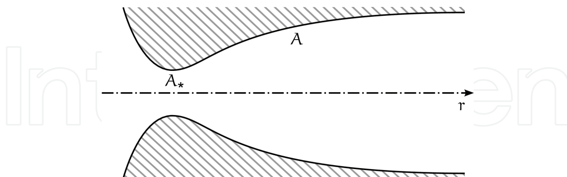
Figure 2. Sketch of a de Laval nozzle. A denotes the local cross-sectional area with the minimum value A_* at its throat position.
