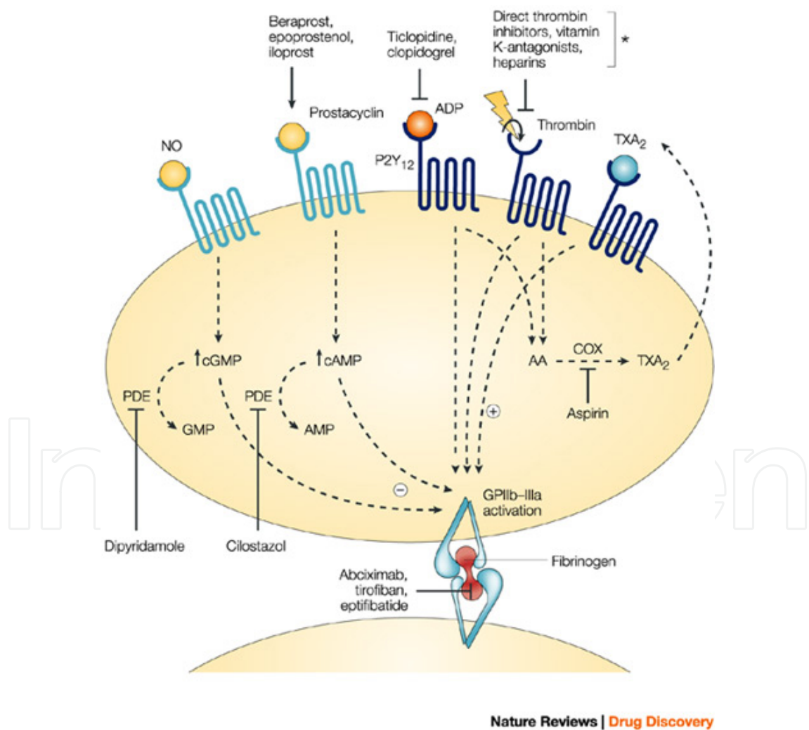
Figure 3. Regulatory pathways of platelets including their stimuli and pharmacologic inhibitors. Reprinted with permission from Macmillian Publishers Lt: Nature Reviews Drug Discovery, Copyright 2003 [85].
