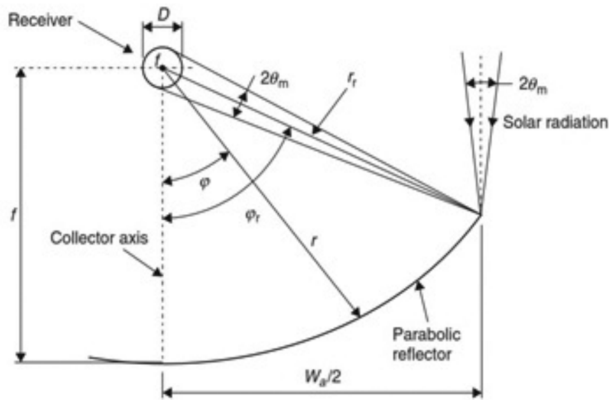
Figure 2. Parabolic trough solar concentrator.
