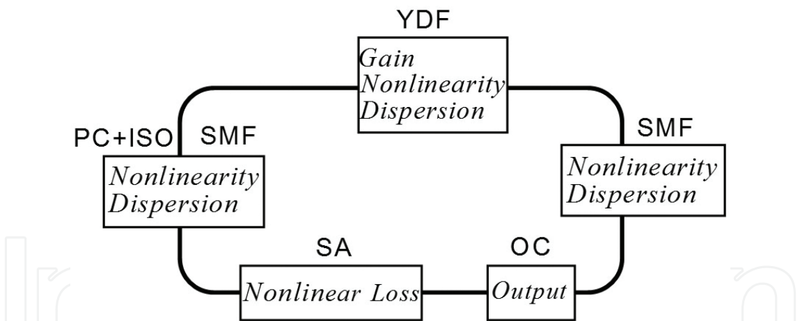
Figure 3. Proposed model of passively mode-locked fiber laser. YDF, ytterbium-doped fiber; SMF, single mode fiber; OC, output coupler; SA, saturable absorber.
