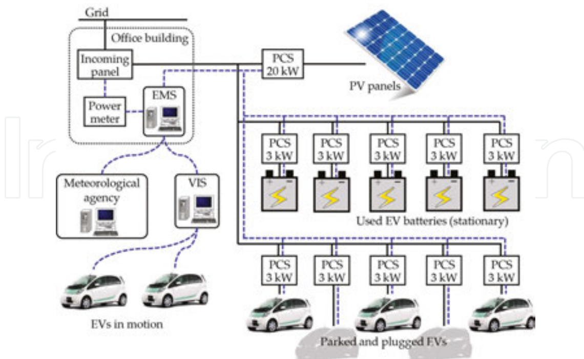
Figure 8. Schematic diagram of the developed test bed.
