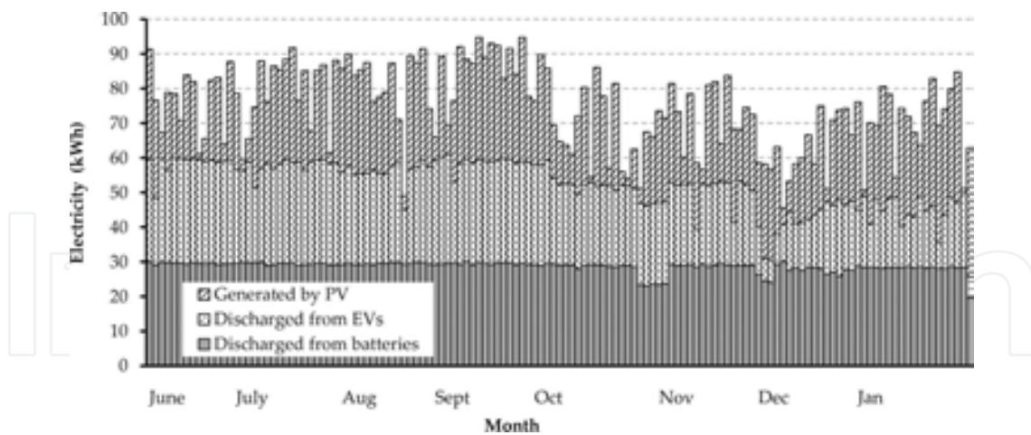
Figure 12. The amount of load leveling in a day by each component (PV, EVs, and used EV batteries).
