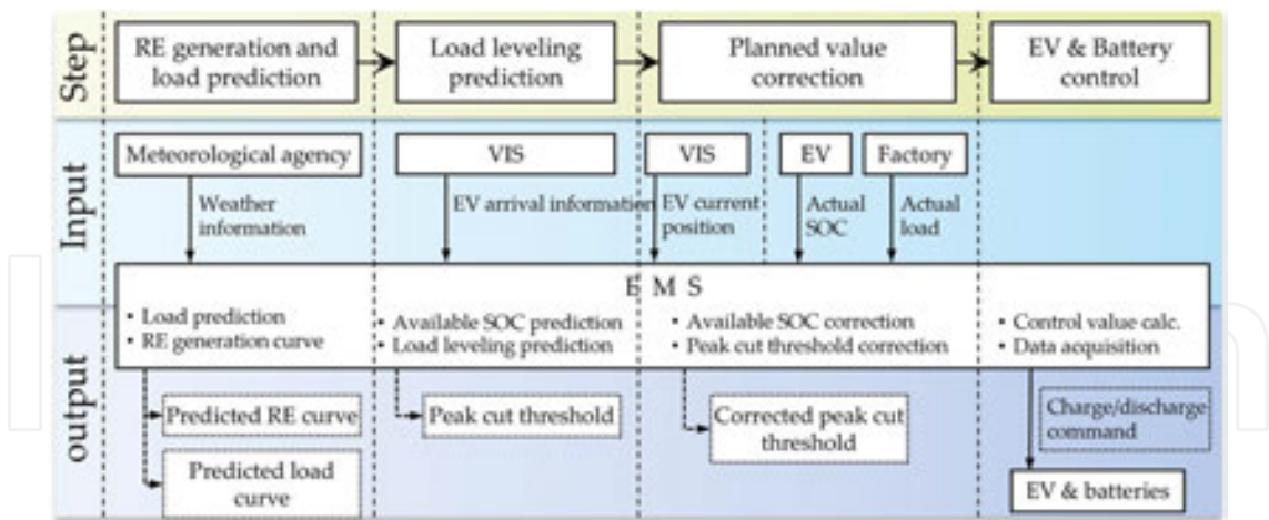
Figure 7. Developed load leveling concept utilizing EVs and their used batteries.
