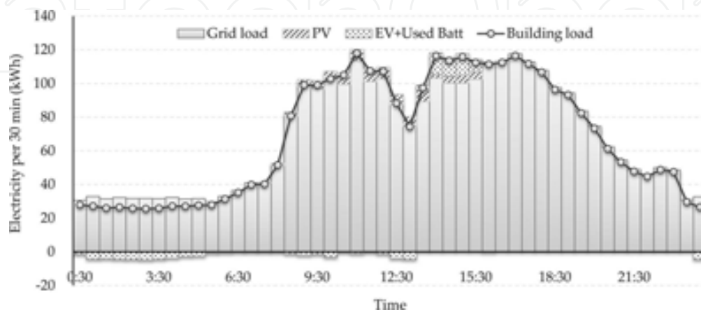
Figure 11. Results of load leveling test during weekdays.
