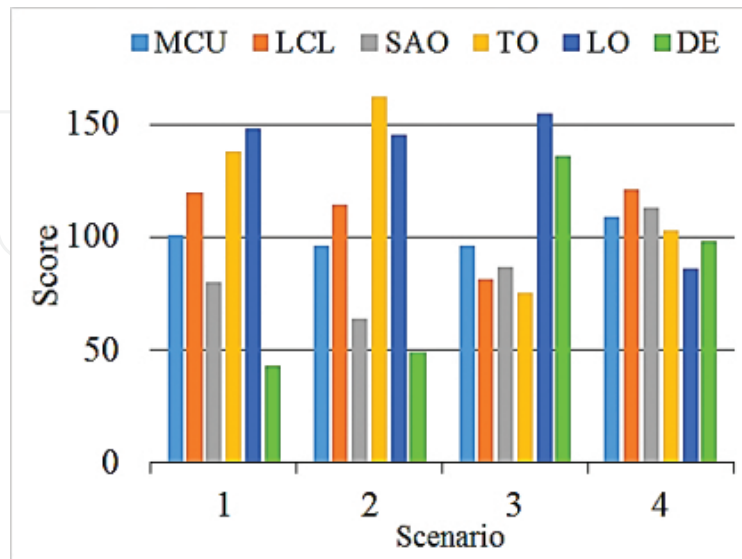
Figure 3. Activity analysis of dependent variables for strata movement based on NNC-based sensitivity analysis results [1].
