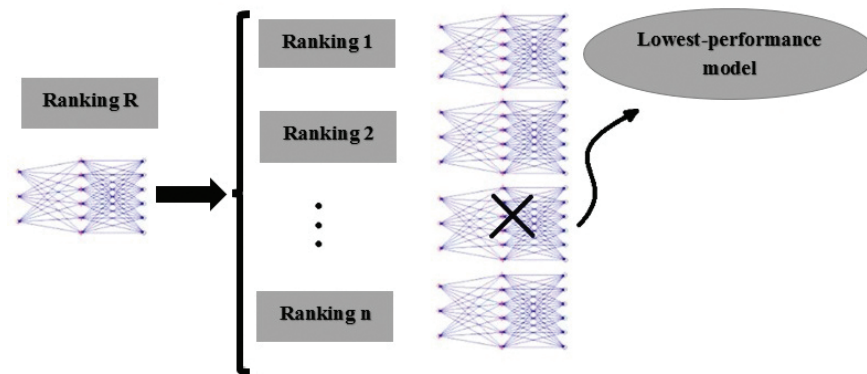
Figure 1. A schematic diagram of NNC-based sensitivity analysis strategy.
