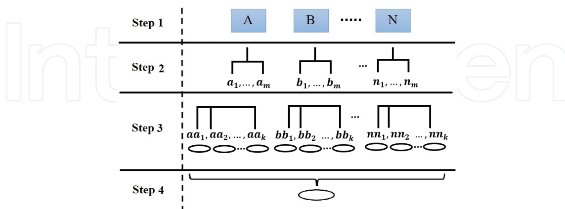
Figure 2. NNC-based sensitivity analysis strategy stepwise procedure: A–N, the neural network model seeds; a_1 - a_m , b_1 - b_m , and n_1 - n_m , the candidate groups of neural network models; aa_1 - aa_k , bb_1 - bb_k , and nn_1 - nn_k , the superior neural network models; ellipse refers to a sensitivity analysis ranking of an input parameter.
