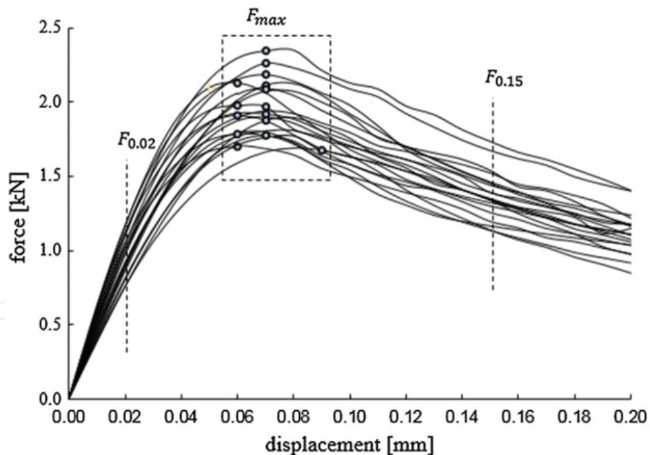
Figure 6. Force-displacement curves at the notch tip S from 20 simulated realizations of notched concrete beams [4].
