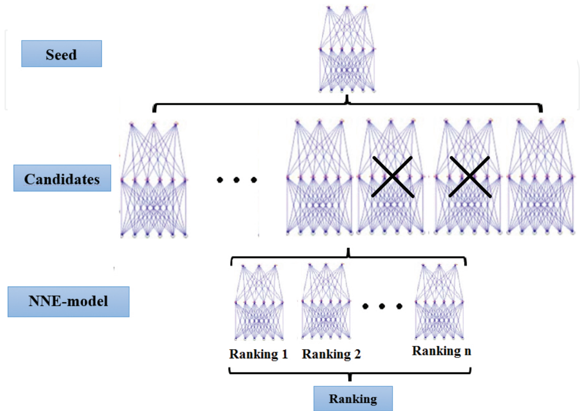
Figure 4. A schematic representation of NNE-based parameter sensitivity analysis.
