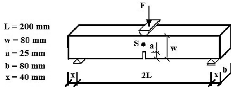
Figure 5. Notched concrete beam under three-point bending [4].
