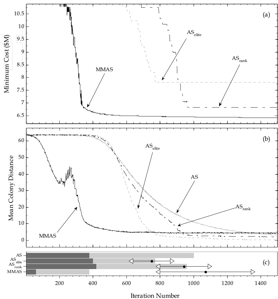
Figure 6. Plots of (a) the minimum cost ($M) found in each iteration f_{min}(t) , (b) the mean colony distance d_{\Sigma}(t) , and (c) run-time statistics for AS, AS_{elite} , AS_{rank} , and MMAS applied to the Hanoi Problem. Plots (a) and (b) are averaged from 20 runs. Plot (c) depicts the three convergence phases: phase-I (dark grey); phase-II (light grey); phase-III (remaining white space). The line graphs overlaying the bar charts in (c) indicate the search-time statistics (based on 20 runs) with the dot indicating the mean search-time, and the left and right arrows indicating the mean minus and plus a standard deviation, respectively
