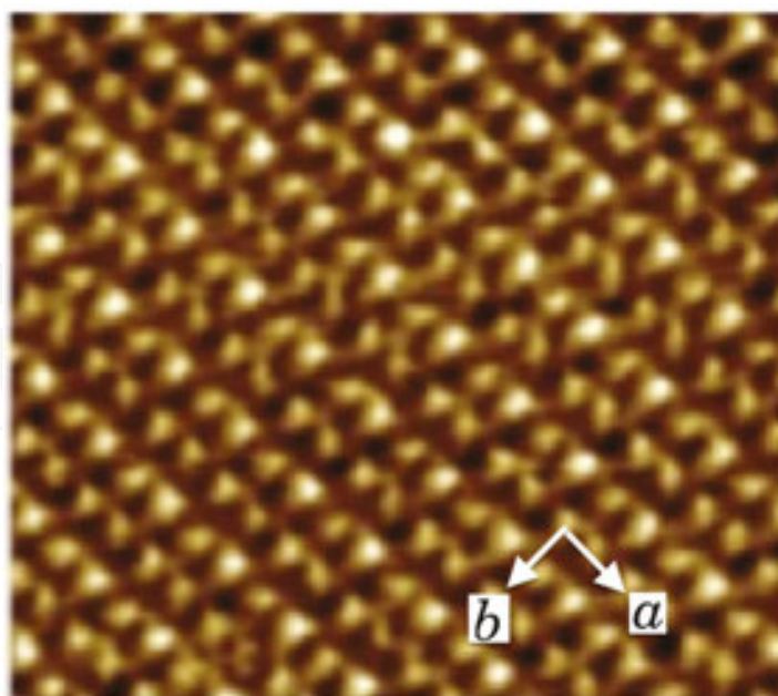
Figure 8. STM image of a thin plate-like single crystal of \alpha\text{-(BEDT-TTF)}_2\text{I}_3 in \approx 7.0 \times 6.5 \text{ nm}^2 , where the thermal drift was corrected with the reported lattice parameters [23]. The assigned a and b axes are indicated by the arrows (reused from Ref. [1]).
