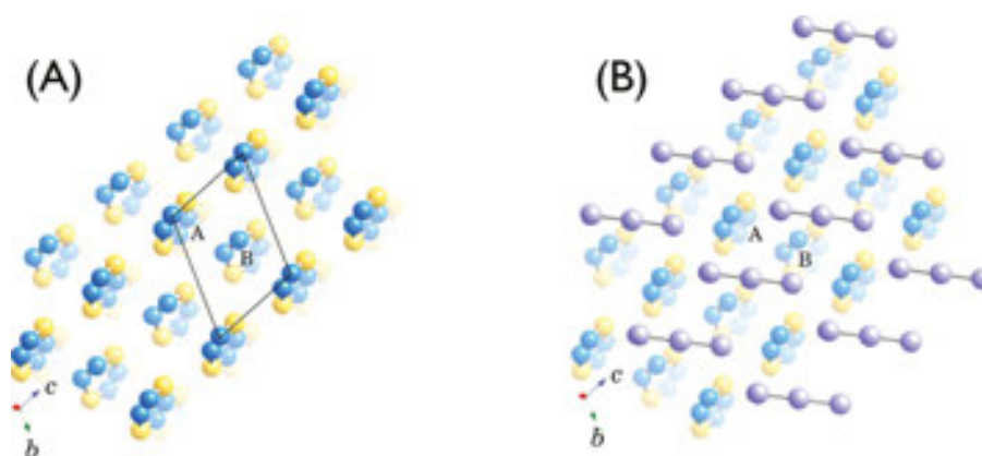
Figure 11. Crystal structure of \beta -(ET) 2 I 3 in the b - c plane at RT [24]. Crystal data are triclinic with a = 15.243 , b = 9.070 , c = 6.597 Å, \alpha = 109.73^\circ , \beta = 95.56^\circ , \gamma = 94.32^\circ . Blue and yellow balls indicate carbon and sulfur atoms, respectively. Hydrogen atoms are not indicated. The unit cell contains two ET molecules, ET(A) and ET(B), and one I 3 - ion. (B) shows relative location of I 3 - ions against ET molecules. Note that the steric hindrance of the I 3 - ions with ET(B) is stronger than with ET(A) in this surface and vice versa in the next layer of I 3 - ions.
