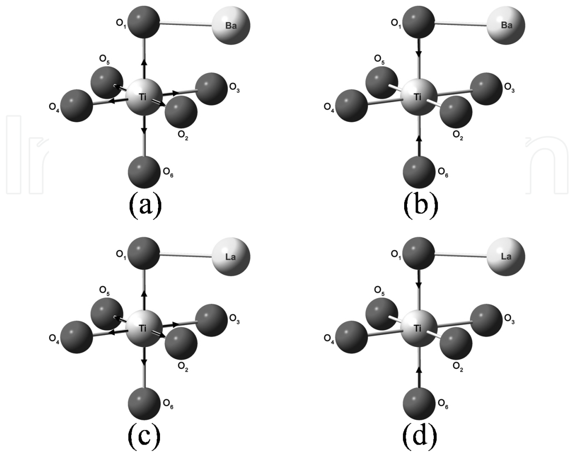
Figure 3. (a) represents the [\text{BaTiO}_3]_2 fragment with the Ti atom fixed in the space and Ti atom being moved 0.003 \text{ \AA} in the direction to \text{O}_1 , \text{O}_2 , \text{O}_3 , \text{O}_4 , \text{O}_5 , and \text{O}_6 atoms and Ba atom and all O atoms are fixed; (b) represents the [\text{BaTiO}_3]_2 fragment with the bond lengths \text{Ti}-\text{O}_1 and \text{Ti}-\text{O}_6 shortened from 0.003 \text{ \AA} ; (c) represents the [\text{LaTiO}_3]_2 fragment with the Ti atom fixed in the space and Ti atom being moved 0.003 \text{ \AA} in the direction to \text{O}_1 , \text{O}_2 , \text{O}_3 , \text{O}_4 , \text{O}_5 , and \text{O}_6 atoms and La atom and all O atoms are fixed; and (d) represents the [\text{LaTiO}_3]_2 fragment with the bond lengths \text{Ti}-\text{O}_1 and \text{Ti}-\text{O}_6 shortened from 0.003 \text{ \AA} .
