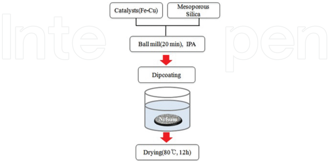
Figure 6. Deposition of catalysts and mesoporous SiO 2 on Ni foam.
