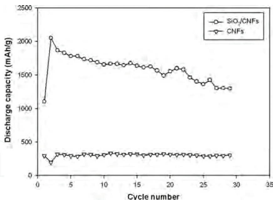
Figure 15. Discharge capacity of CNFs and \text{SiO}_2/\text{CNF} composite.
