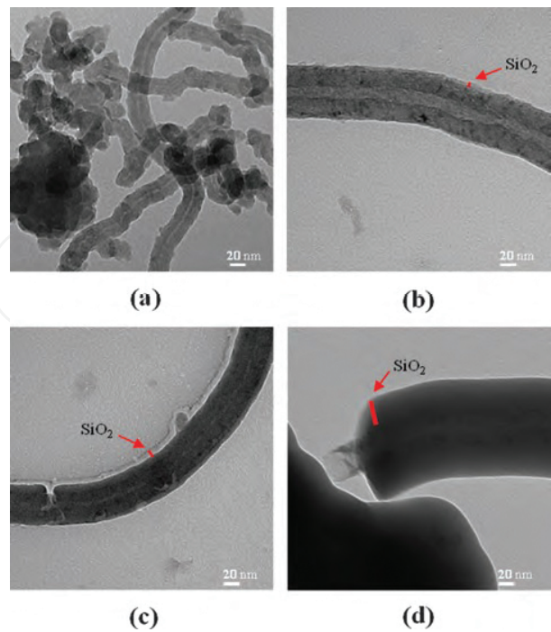
Figure 14. TEM images of CNFs (a) and SiO 2 /CNF composite (b)–(d).
