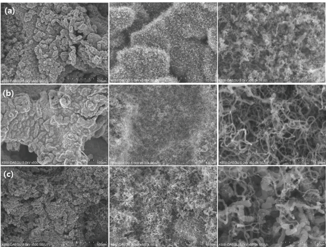
Figure 9. SEM images of CNFs and mesoporous SiO 2 -CNF composites. (a) CNF-BF/Fe-Cu/Ni foam, (b) CNF-BF/Fe-Cu/mesoporous SiO 2 /Ni foam, and (c) CNF-BF/mesoporous SiO 2 /Ni foam.
