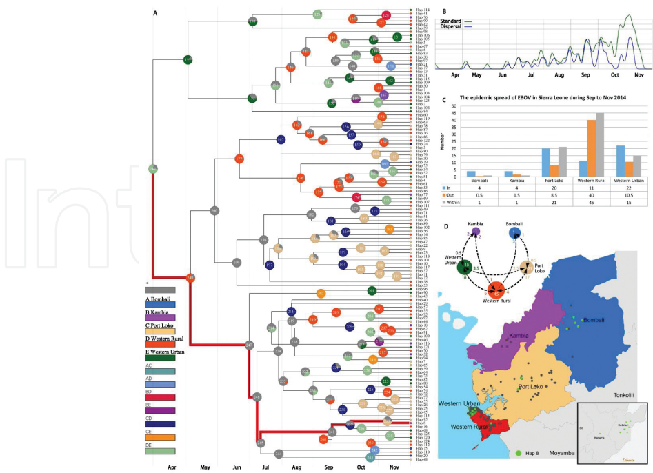
Figure 5. Phylogeographic analysis of the epidemic spread of Ebola virus in Sierra Leone. (A) Results of the biogeographic analysis of haplotypes using S-DIVA method. Pie charts show the probability values of the ancestral areas reconstructed at each node. Areas are colour-coded as in the legends allowing for single or combined distributions. (B) The diagram of dispersal events (blue line) and node density (green line) (C) The total number of immigration (in), emigration (out) and the divergence (within) of haplotype of each districts (D) The circle represented the number of dispersals among Bombali, Kambia, Port Loko, Western Rural and Western Urban. Map to show the geographical distribution of the districts of EBOV from September to November 2014. The distribution of Hap8 was highlighted with green points. We obtained the boundary data of the District from the GADM database of Global Administrative Areas version 2.0 ( http://www.gadm.org ), and the map was created in ArcGIS 9.2 software (ESRI Inc., Redlands, CA, USA).
