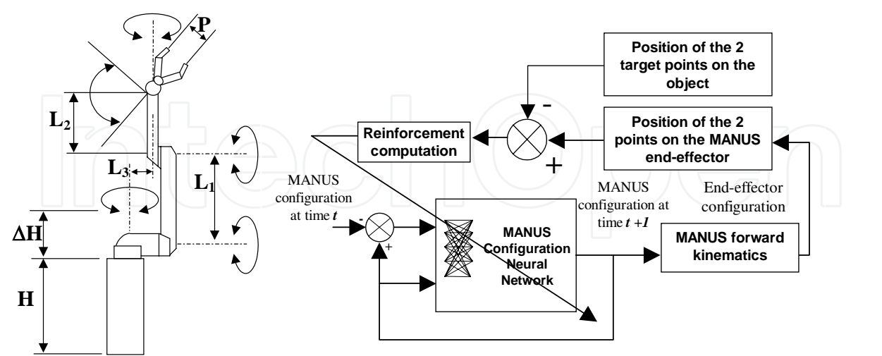
Fig. 11. a/ Degrees of freedom of the MANUS robot , b/ Model architecture.
