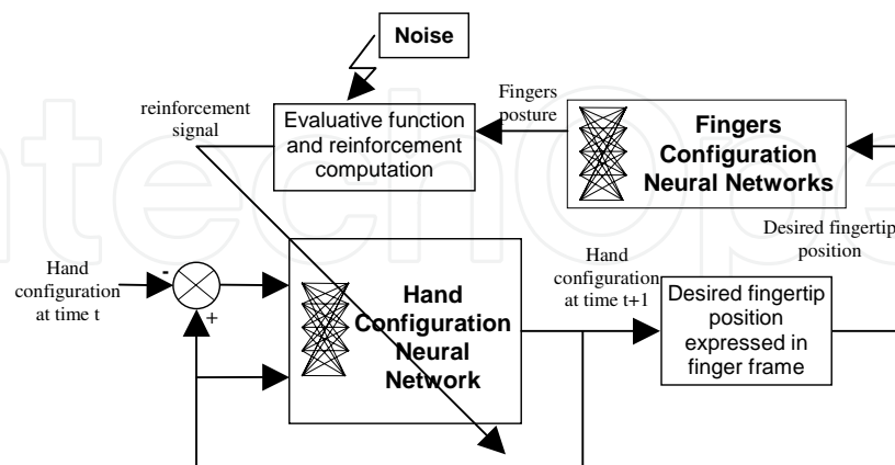
Fig. 2. Model architecture.
