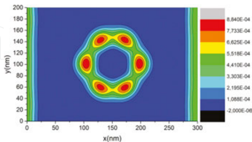
Figure 11. Contour plot of the charge distribution obtained from the Hartree-Fock calculation in multiples of 10^{14}\text{cm}^{-2} for a magnetic field of B = 2.5 Tesla. In this regime, the electron system appears fully spin polarized.
