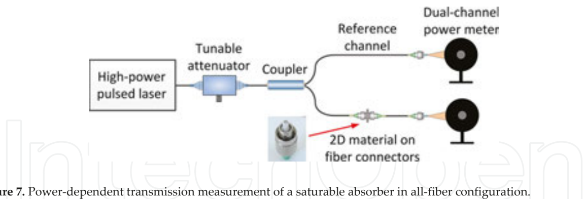
Figure 7. Power-dependent transmission measurement of a saturable absorber in all-fiber configuration.
