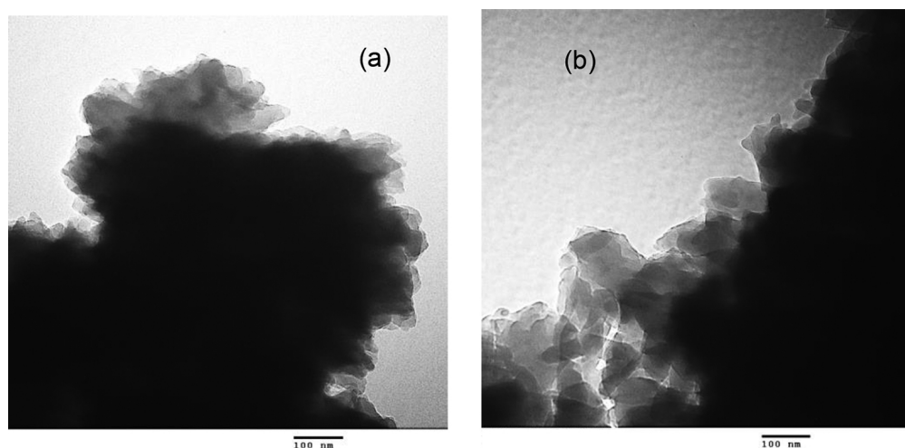
Figure 10. TEM micrographs of (a) PANI-10% \text{WS}_2 , (b) PANI-64% \text{WS}_2 .
