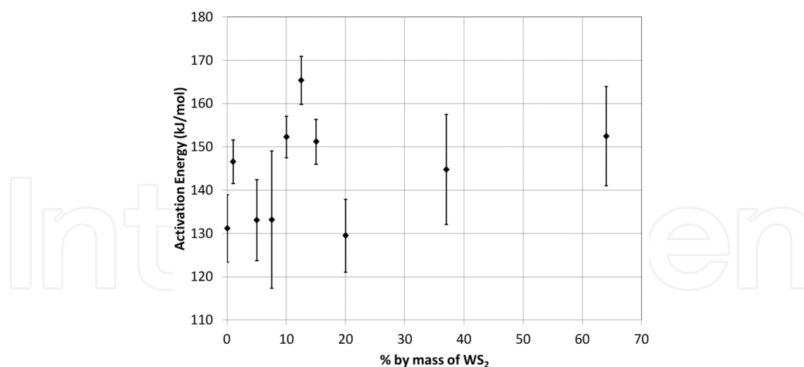
Figure 12. Plot of activation energy values versus mass% of \text{WS}_2 .
