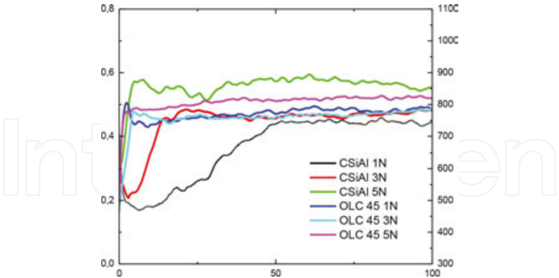
Figure 9. Comparative view of the friction coefficient of substrate (OLC45) and of CSiAl film deposited on the substrate at different loading forces.
