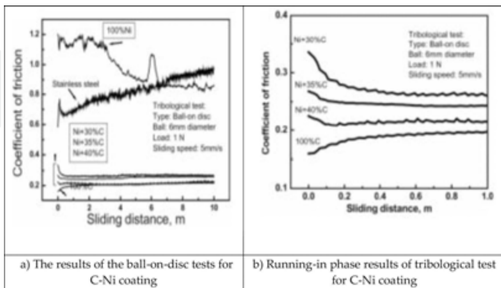
Figure 5. Frictional behavior of C-Ni coatings.
