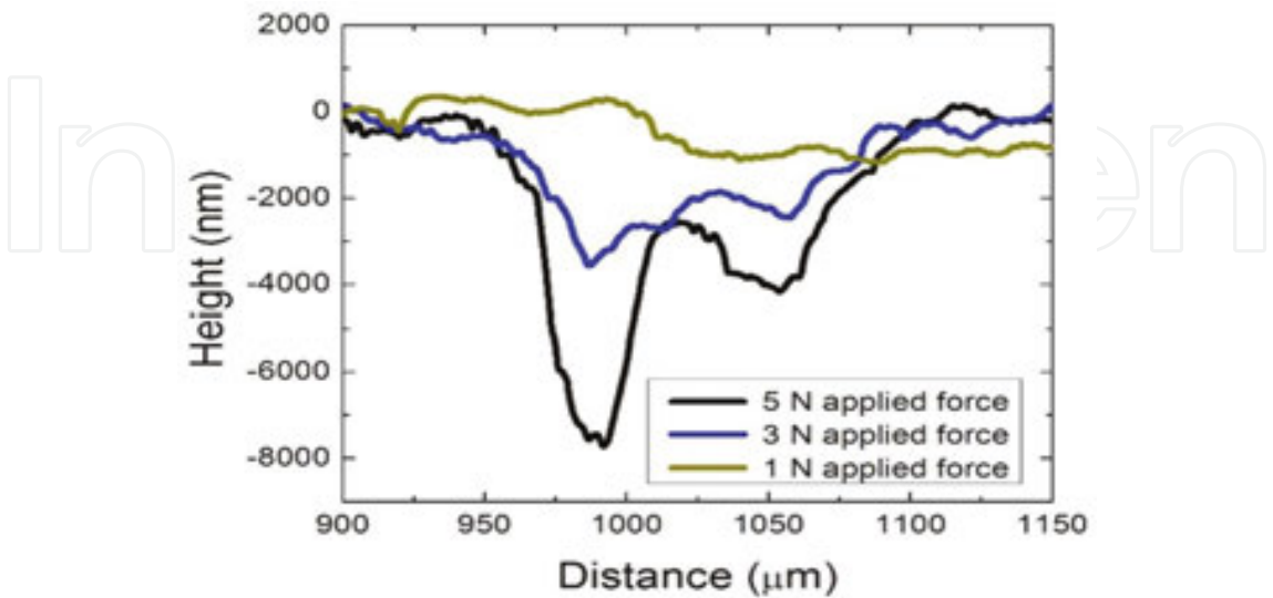
Figure 10. Depth profile of the wearing traces after tribological characterization.
