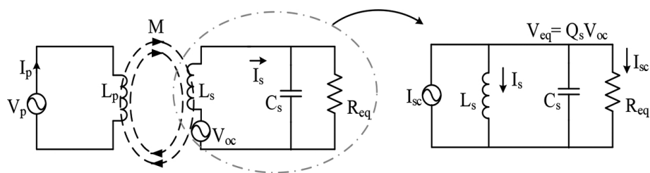
Figure 12. Simplified circuit with a parallel-tuned secondary.
