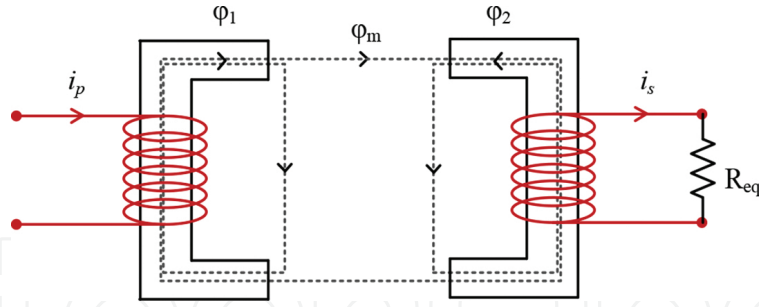
Figure 2. Typical flux linkage in an ICWPT system.
