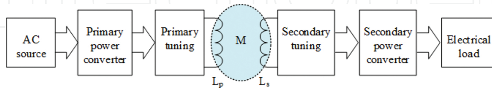
Figure 3. Fundamental elements of an ICWPT system.
