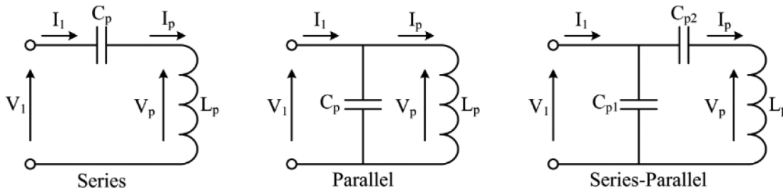
Figure 4. Primary tuning topologies.
