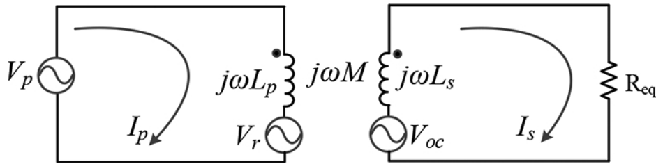
Figure 7. Frequency domain mutual inductance model.
