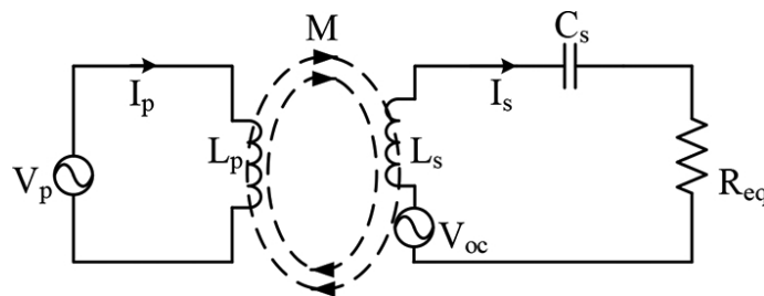
Figure 11. Simplified circuit with a series-tuned secondary.
