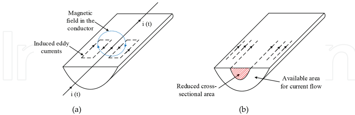
Figure 9. Impact of skin effect on the coil ESR: (a) generated eddy currents and (b) reduced cross-sectional area due to skin effect.
