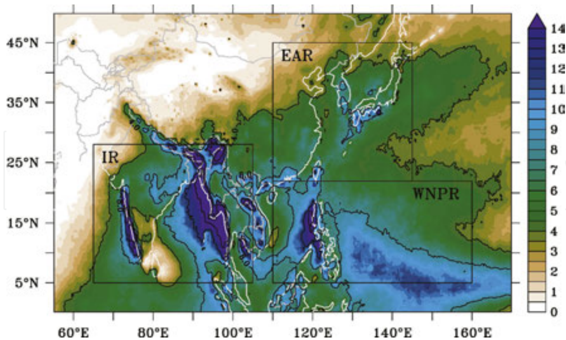
Figure 1. Mean May–August precipitation (mm day −1 ) from GPCP [40] daily data (1997–2007), and an illustration of the three main domains used for this study: EAR(22°–45°N, 105°–145°E), IR(5°–28°N, 70°–105°E), and WNPR (5°–22°N, 105°–160°E).
