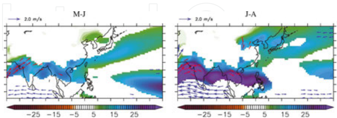
Figure 8. Change in 850 hPa moisture flux (shading, \text{g kg}^{-1} \text{ m s}^{-1} ) and winds (vectors, \text{m s}^{-1} ), averaged over MJ and JA. For the winds, the vectors are plotted only for a change larger than 0.5 \text{ m s}^{-1} , and red (blue) indicates positive (negative) changes. For the moisture flux, only values that exceeded a 90% confidence level with a two-tailed Student’s t test are shaded.
