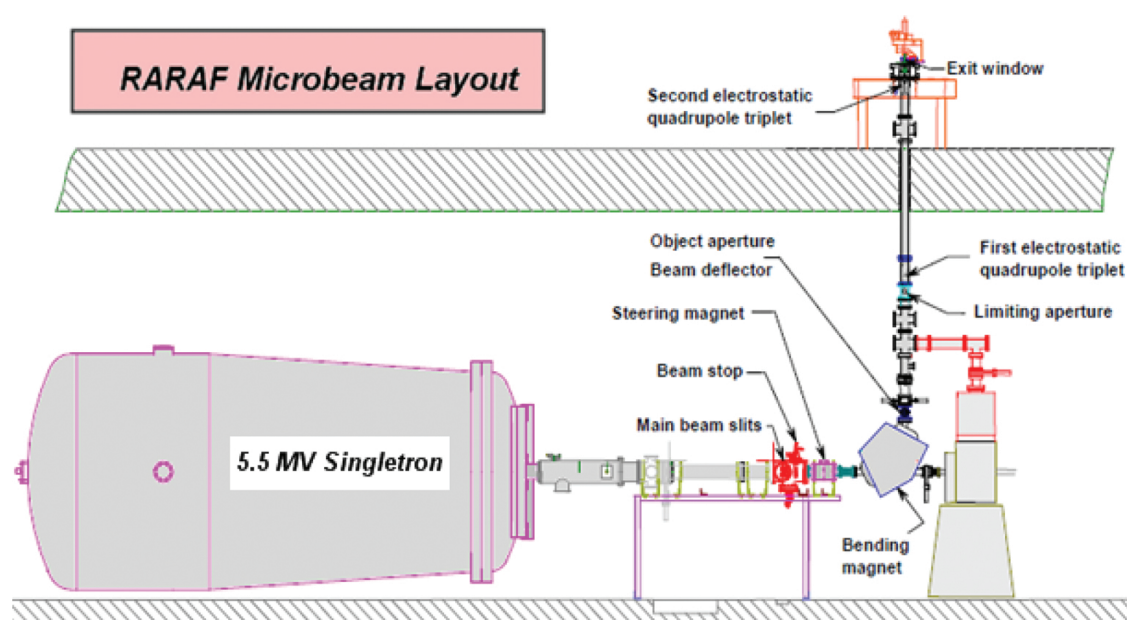
Figure 1. RARAF microbeam.
