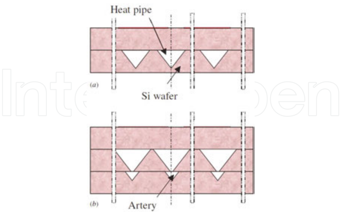
Figure 8. Transverse cross-sections of a MHP array (a) with triangular channels and (b) with triangular channels coupled with arteries [36].
