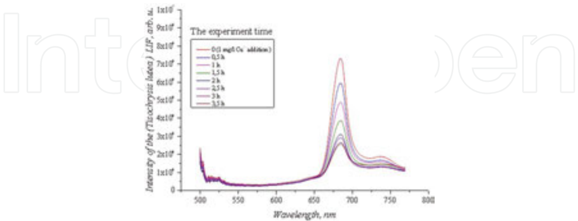
Figure 14. The fluorescence spectra of micro-algae Tisochrysis lutea under the influence of copper ions at a concentration of 1 MPC.
