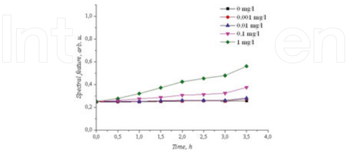
Figure 17. Dependence of the spectral feature of micro-algae Tisochrysis lutea from time under the influence of copper ions.
