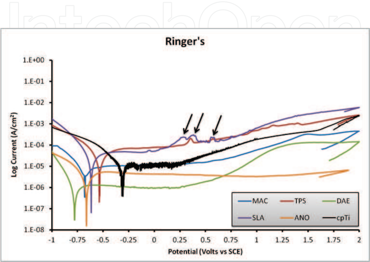
Figure 5. Anodic scans from dental implants with different surface modifications. Oxidation peaks (pointed by black arrows) were identified for TPS and SLA. All the surfaces showed a breakdown potential ( E_{\text{pit}} ) and negative hysteresis in reverse scanning (a small part of reverse scanning curve at 2 V is appeared for all materials).
