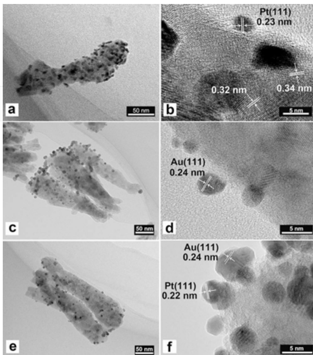
Figure 13. TEM images and HRTEM images of (a–b) Pt/TiO 2 NRAs coated with 10 cycles; (c–d) Au/TiO 2 NRAs coated with 10 cycles; (e–f) Au/Pt/TiO 2 NRAs.
