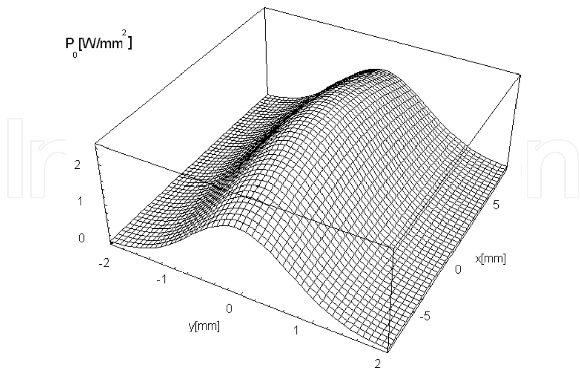
Figure 5. The simulated intensity in the cross section of the beam delivered by ALIN-10.
