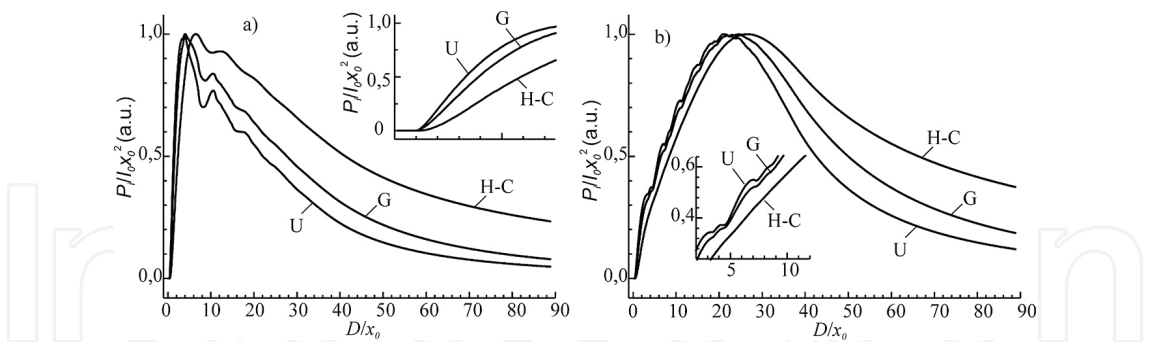
Figure 15. Modulation characteristics of a IMFODS with a) alternating linear configuration of transmitting and receiving fibres; b) semicircle configuration of emitting and receiving fibres. U – uniform irradiance function; G – Gaussian irradiance model; H-C – He-Cuomo theoretical irradiance function.
