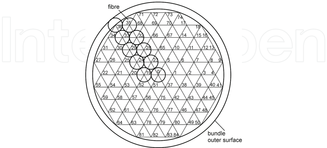
Figure 14. Three bundle configurations were modelled The numbers denote the centres of individual fibres.
