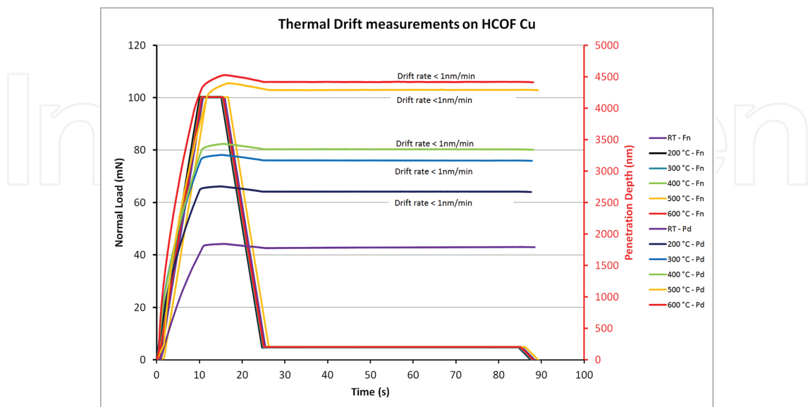
Figure 4. Thermal drift of the measuring system registered under various loads and temperatures.
