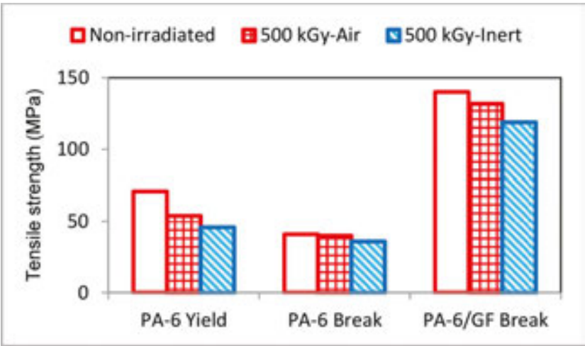
Figure 22. Comparison of variations of tensile strength for virgin PA-6 and composite PA-6/GF \gamma -irradiated by 500 kGy dose.
