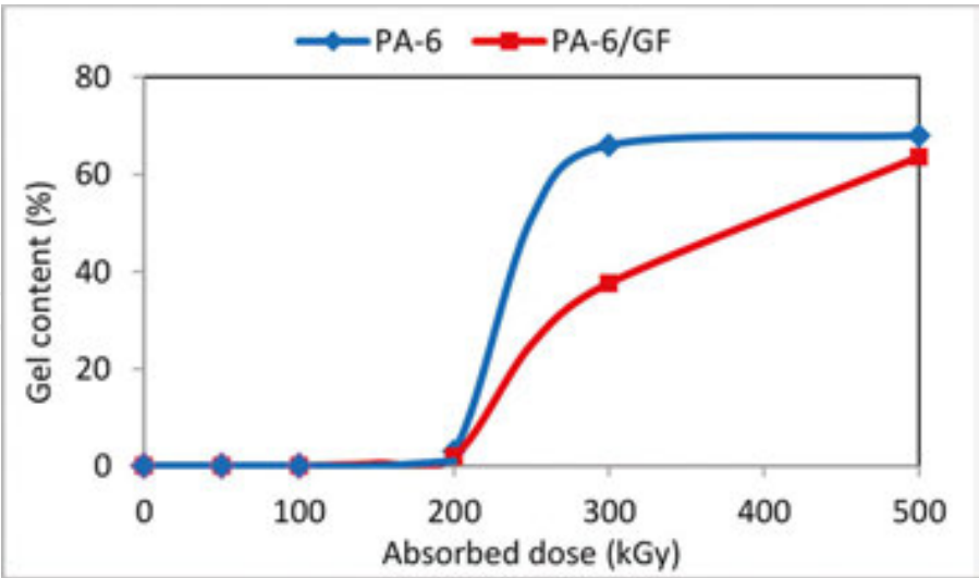
Figure 2. Dependence of gel content on absorbed electron beam dose for virgin PA-6 and PA-6/GF (30%) composite [7]. With permission of Elsevier.
