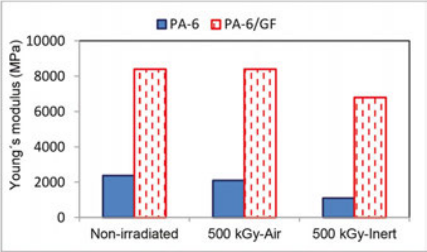
Figure 21. Comparison of variations of Young’s modulus for virgin PA-6 and composite PA-6/GF \gamma -irradiated by 500 kGy dose.
