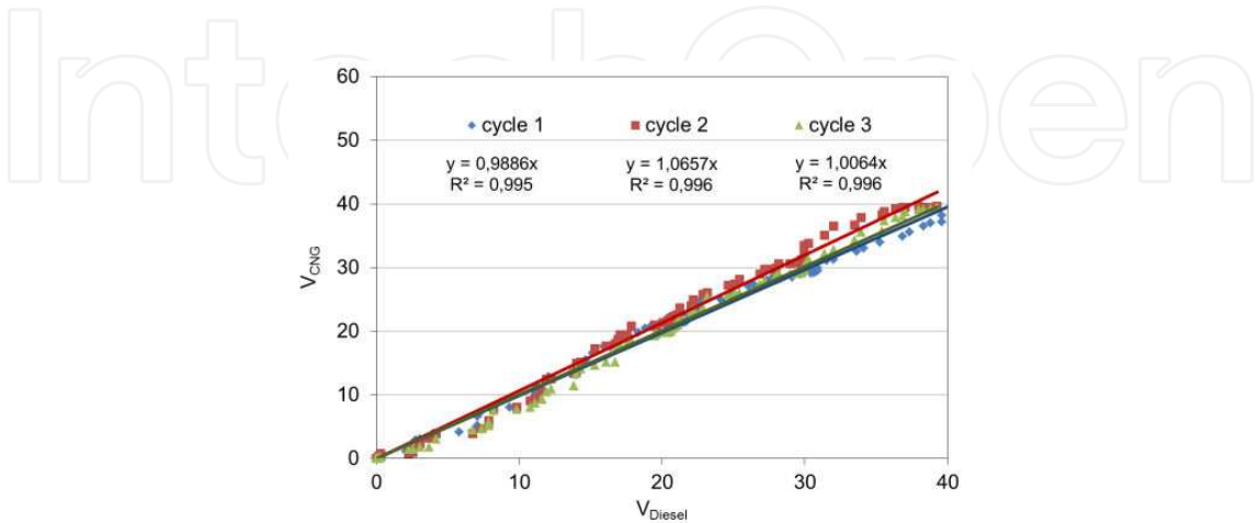
Figure 9. Comparison of speeds of vehicles in subsequent trials of SORT 1 cycles(time compliance allowed for).
