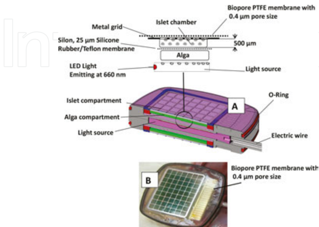
Figure 8. The photosynthetic bioartificial pancreas. The device has a core illumination panel directing the 660 nm light to both sides. The algae chamber is laid directly on the illumination panel and is separated from the islet chamber with gas-permeable thin silicone/Teflon membrane. The islet chamber is protected from the immune cells by porous biopore membrane. Panel A: Detailed cross-section of the device. Panel B: Actual view of the device.
