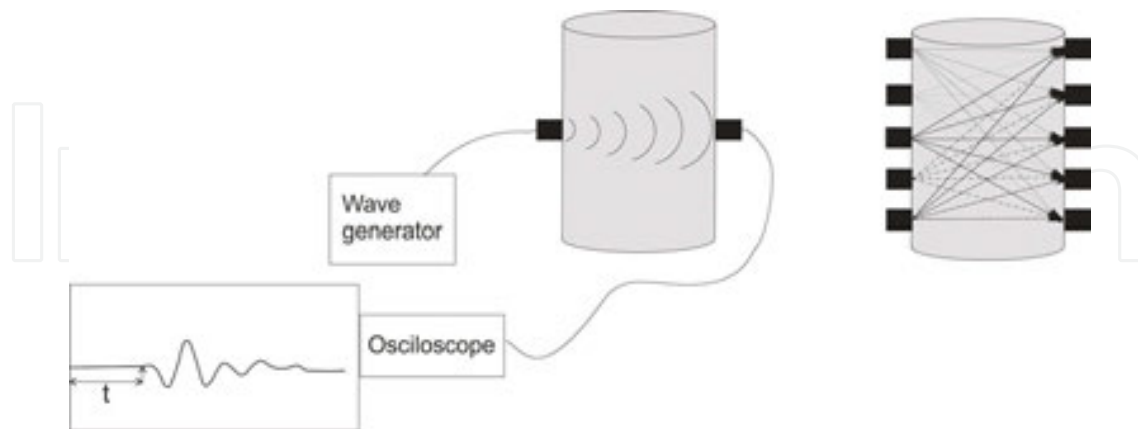
Figure 11. System for measuring wave velocity (left), to do acoustic tomography (right).
