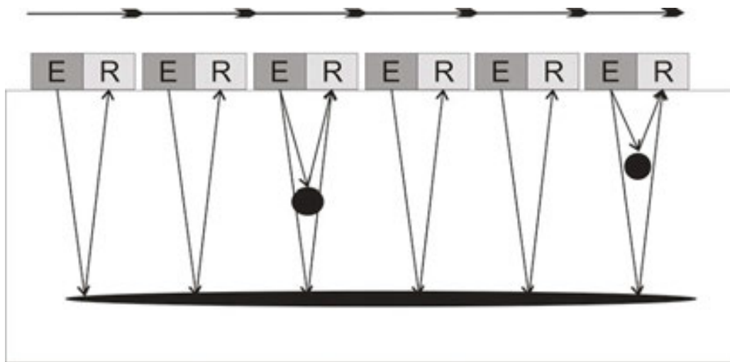
Figure 18. Principle of ground penetrating radar (GPR).
