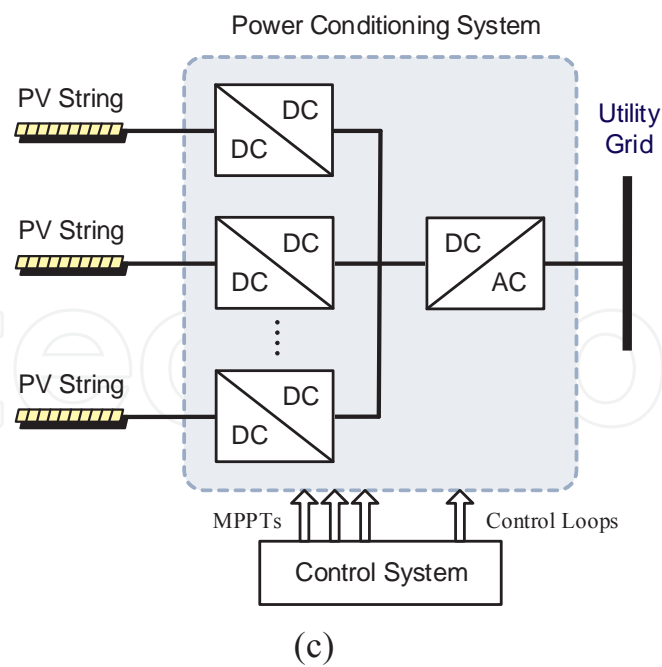
Figure 4. PV PCS configurations: (a) single-stage inverter, (b) dual-stage inverter, and (c) multi-stage inverter.
