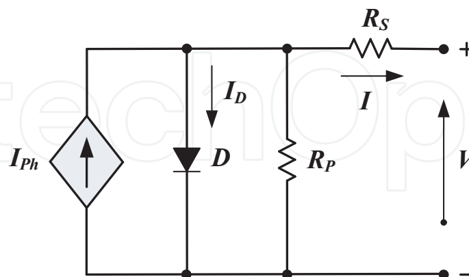
Figure 1. Equivalent circuit of a PV cell
