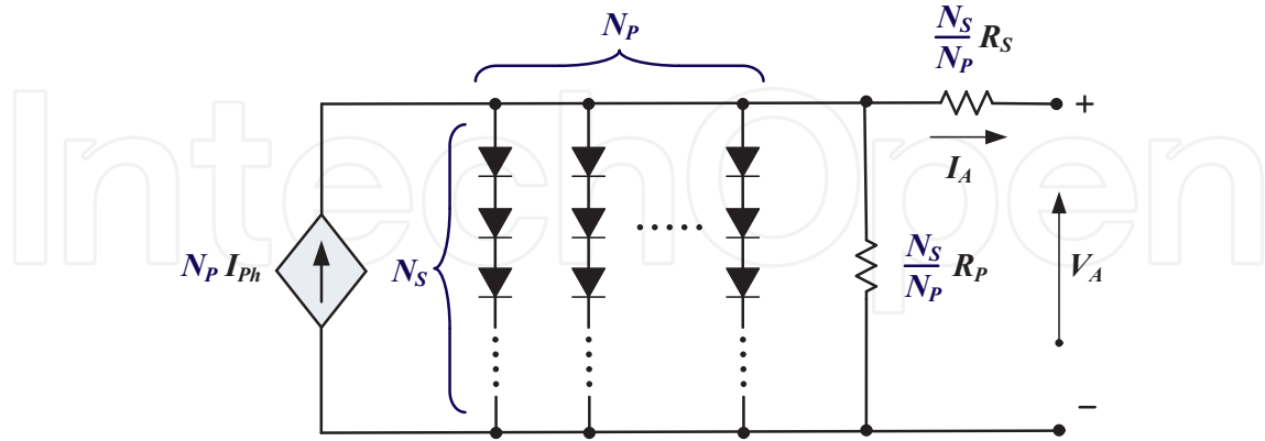
Figure 2. Equivalent circuit of a generalized PV generator
