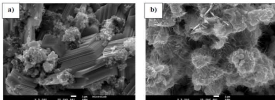
Figure 4. FEG-SEM images for (a) as-deposited and (b) annealed Zn-TiO 2 nanocomposite films [72].
