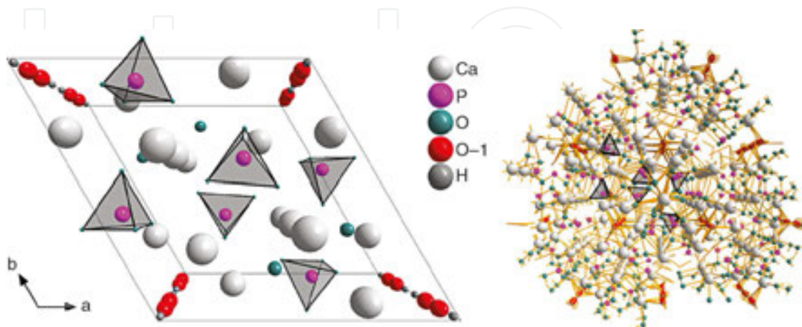
Fig. 16. Crystallographic structure of human dental enamel apatite (perspective view along the c-axis): P6_3/m , a = 9.4081 \text{ \AA} , b = 6.8887 \text{ \AA} , c:a = 0.7322 and V = 528.05 \text{ \AA}^3 [121].
