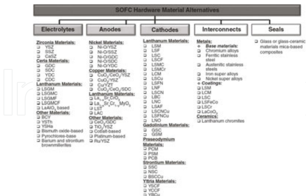
Fig. 9. Comprehensive list of various materials used in SOFC [77].
