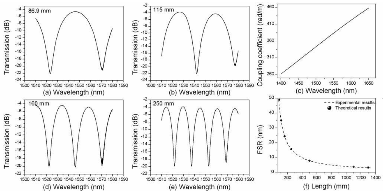
Figure 3. Transmission spectra of TCF-based filters with lengths, L_{\nu} , (a) 86.9, (b) 115, (d) 160, (e) 250 mm, (c) calculated coupling coefficient as a function of wavelength, (f) measured and calculated FSRs for various lengths of TCF.
