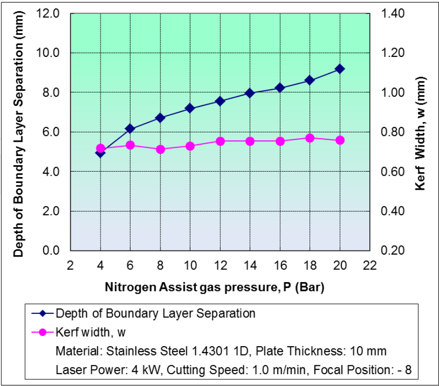
Figure 9. Effect of assist gas pressure on the location of boundary layer separation point and kerf width in inert gas-assisted laser cutting
