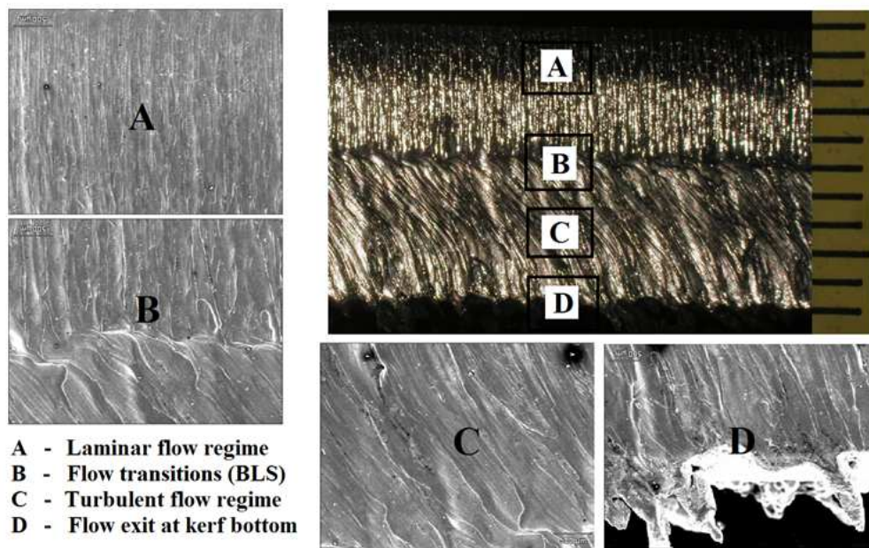
(b) The different flow regimes in the cut kerf
