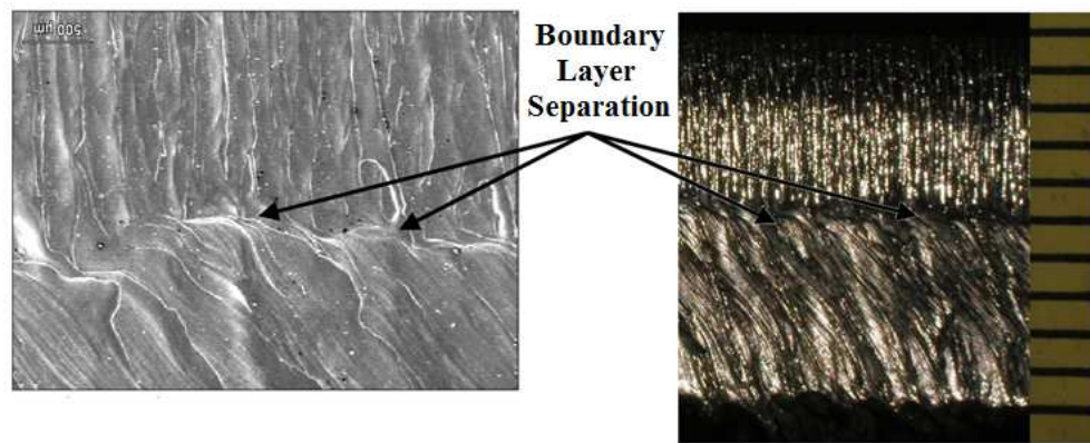
(a) Boundary Layer Separation Point
