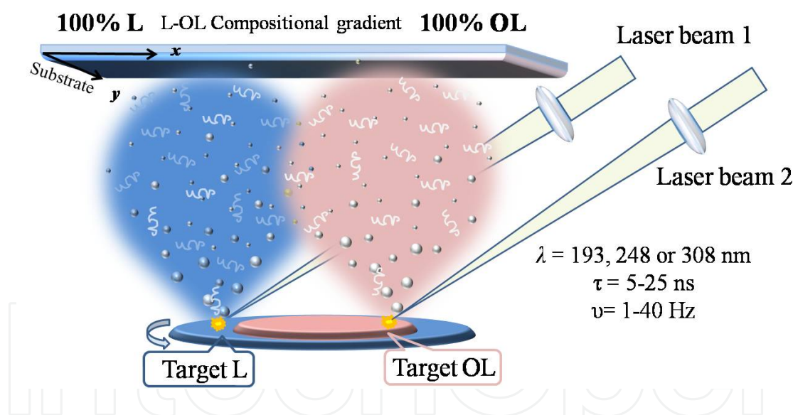
Figure 3. The design of the experimental setup.
