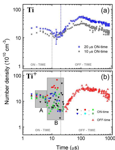
Figure 10. Time-resolved evolution of the Ti (a) and \text{Ti}^+ (b) number density in Ar-Ti HiPIMS discharge measured by ROAS. The A and B time intervals correspond to the density depletion and the current self-organization, respectively. Six independent measurements have been undertaken in the case of \text{Ti}^+ continuously showing the density instabilities in the interval B. Ar pressure = 20 mTorr, z = 5 cm. Reproduced with permission from Britun et al. [38]. Copyright 2015 AIP Publishing.
