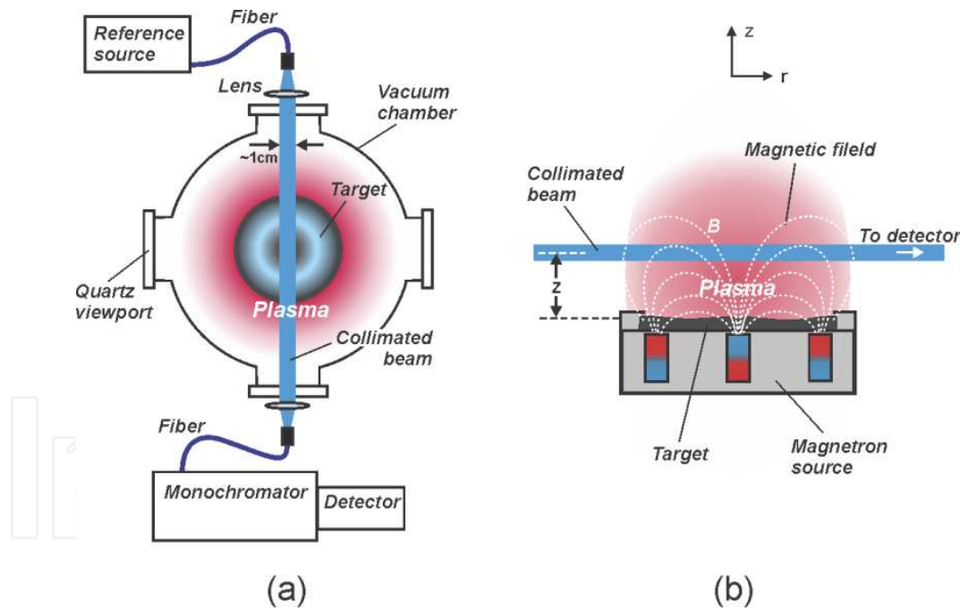
Figure 5. Top (a) and side (b) view of the experimental setup utilized for absolute density measurements in a magnetron sputtering discharge by ROAS. Role of the reference source is played by a hollow cathode lamp. Reproduced with permission from Britun et al. [38]. Copyright 2015 AIP Publishing.
