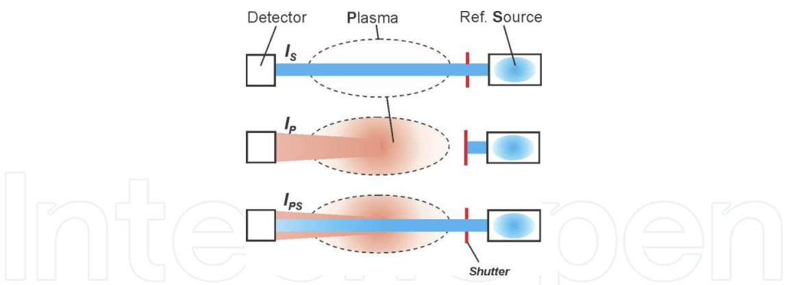
Figure 3. Schematic illustration of the absorption technique and the physical meaning of the quantities I_p , I_s , and I_{ps} .
