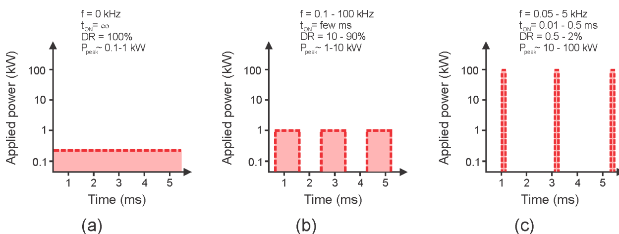
Figure 2. Comparison between the DCMS (a), P-DCMS (b), and HiPIMS (c) magnetron sputtering techniques in terms of the temporal distribution of the applied power. Typical range of the relevant discharge parameters and the values along both horizontal and vertical axes are given for reference only. The quantities f , t_{\text{ON}} , DR, and P_{\text{peak}} stand for repetition frequency, plasma on time, duty ratio, and peak power, respectively.
