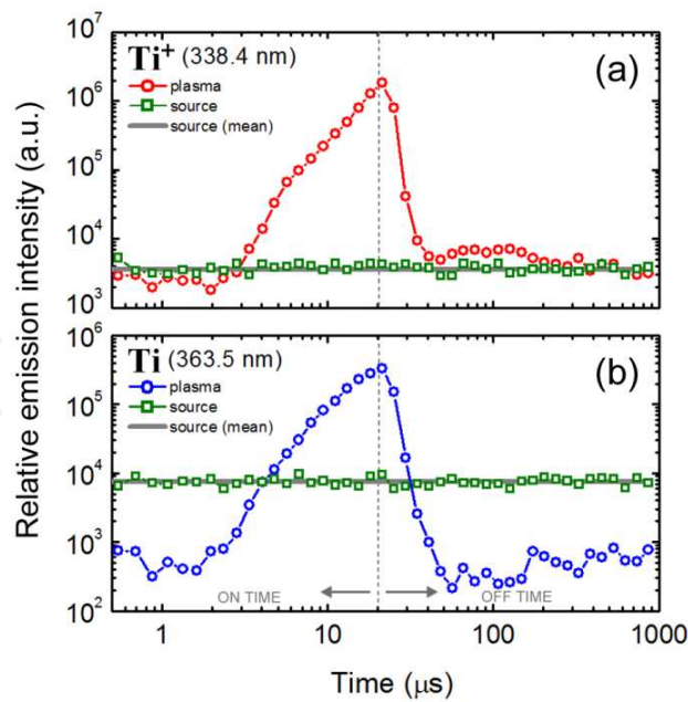
Figure 11. Typical example of the time evolution of Ti + (a) and Ti (b) emission line intensity in Ar-Ti HiPIMS discharge comparing to the intensity of the same emission lines in the reference source (HCL) showing a dramatic increase in the emission intensity at the end of the HiPIMS pulse. Ar pressure = 20 mTorr, z \sim 1 cm.
