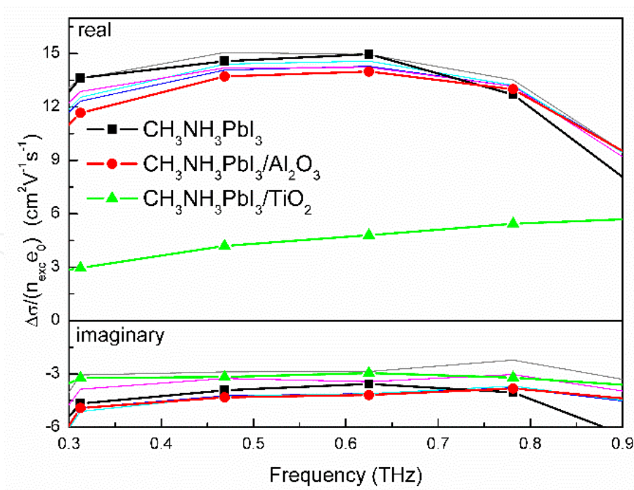
Figure 5. Photoconductivity spectra of MAPbI 3 /Al 2 O 3 at pump-probe delay of 10 ps normalized with n_{exc}e (line with symbols). Solid lines are spectra at 100 ps (blue), 200 ps (cyan), 600 ps (magenta), and 950 ps (gray). (Reprinted with permission from [57], Copyright 2014, American Chemical Society)
