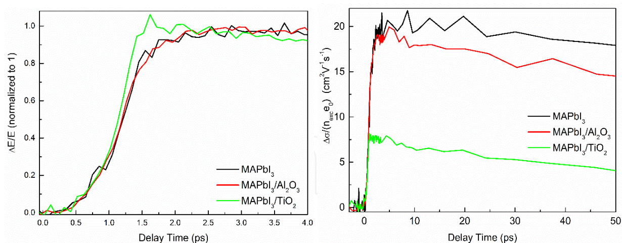
Figure 1. THz photoconductivity kinetics of neat MAPbI 3 , MAPbI 3 /Al 2 O 3 , and MAPbI 3 /TiO 2 . a. Normalized to 1 ( \lambda_{\text{pump}} = 400 nm, I_{\text{exc}} = 1.7 \times 10^{13} ph/cm 2 per pulse), b. Normalized with n_{\text{exc}} . (Reprinted with permission from [57], Copyright 2014, American Chemical Society)
