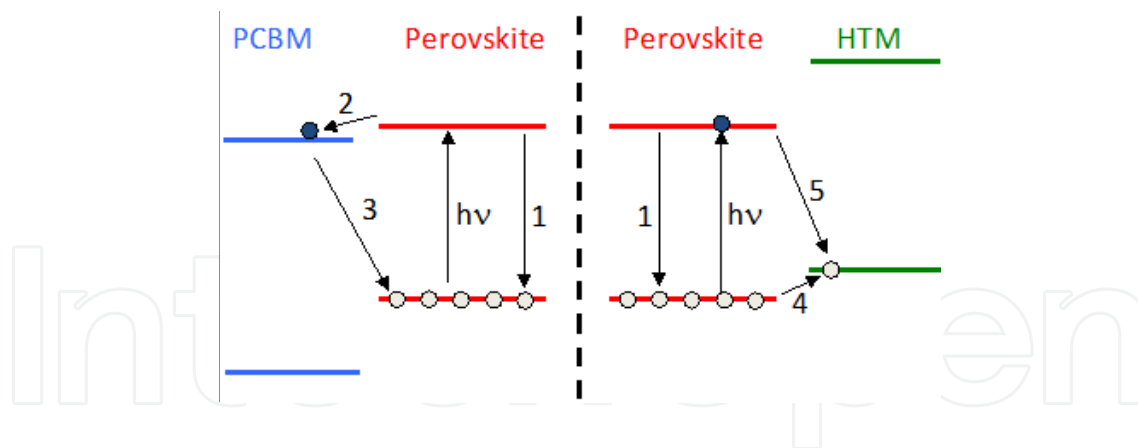
Figure 11. Schematic diagram of injection and recombination dynamics in from neat MAPbI 3 to PCBM and Spiro-OMeTAD.
