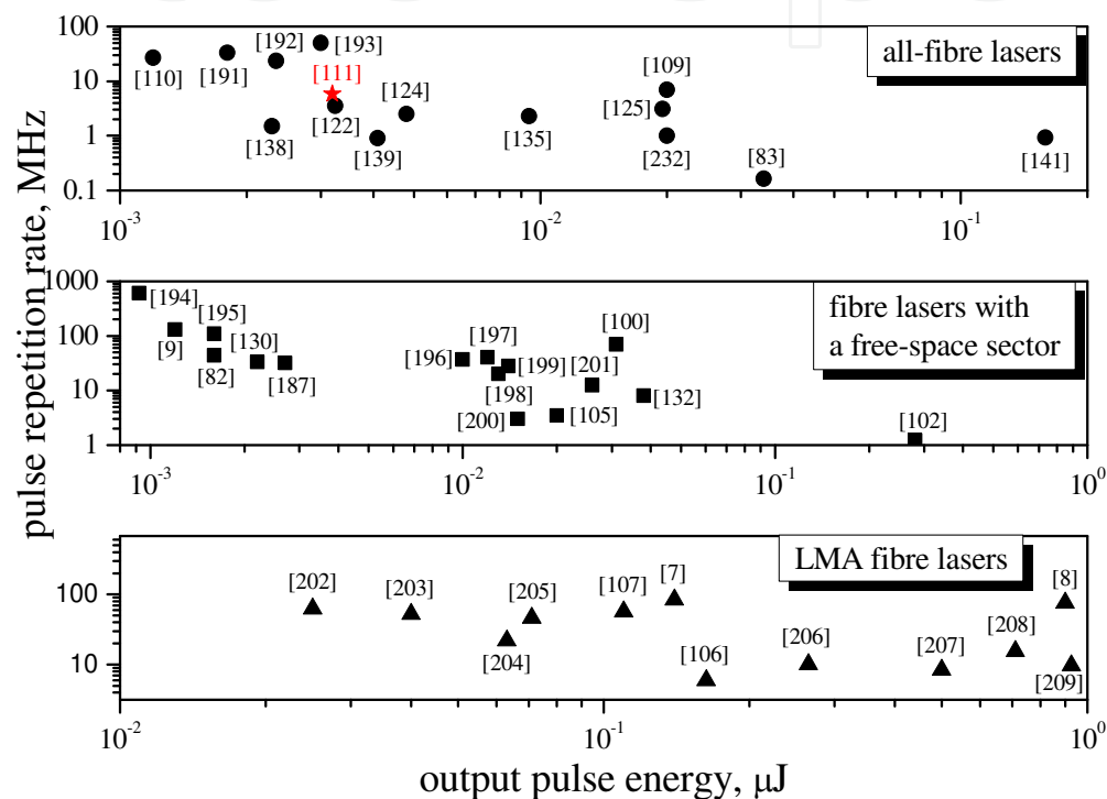
Figure 8. Experimental realizations of DSs in fibre lasers (Refs. [7-9,82,83,100,102,105-107,109-111,122,124,125,130,132,135,138,139,140,141,187,191-209,232]; Ref. [111] corresponds to a DS in the anomalous GDD region).
