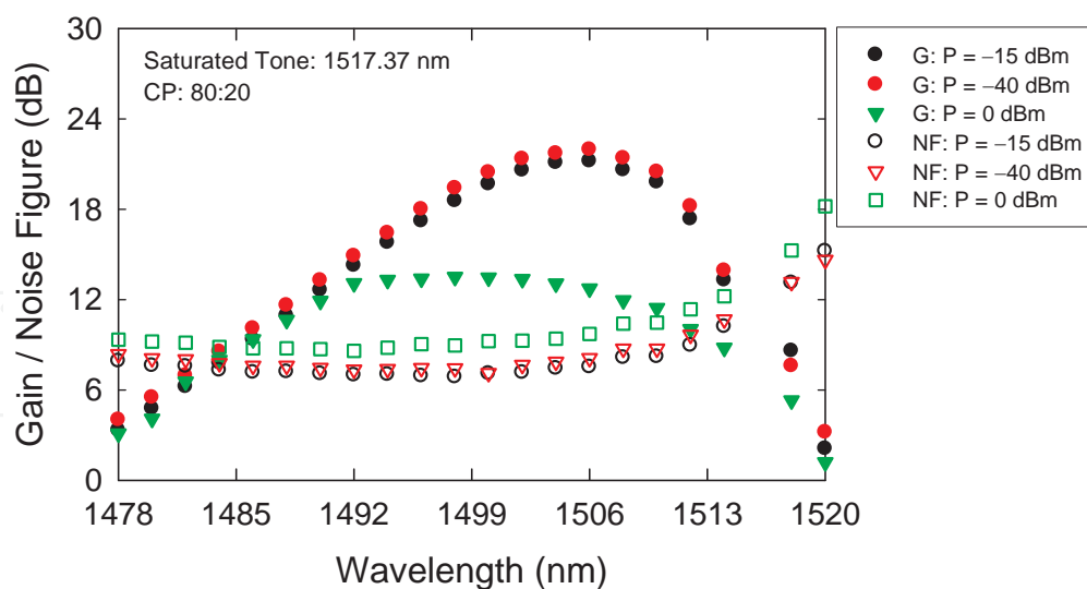
Figure 5. Measured gain and NF spectra of the S band gain-clamped EDFA in the wavelength of 1478–1520 nm with 80% input ratio at the input signal power P = 0 , -15 , and -40 dBm at the lasing wavelength of 1517.37 nm, respectively.
