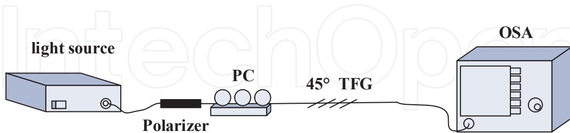
Figure 7. The experiment setup of PER measurement
