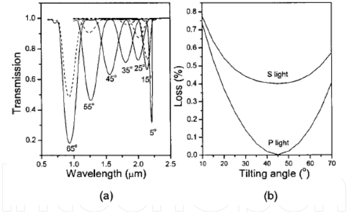
Figure 2. (a) Simulated transmission spectra of TFGs with various tilting angles. TM-light (dashed curves); TE-light (solid curves); (b) simulated transmission losses of TFGs versus tilting angles for s -light (TE) and p -light (TM). The peak wavelength is set as 1.55 \mu\text{m} and the grating period is varied accordingly[6].
