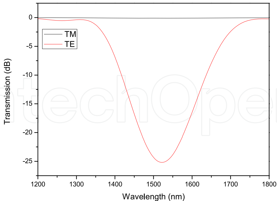
Figure 3. The simulation results of the transmission loss against the wavelength for TM polarization (black line) and TE polarization (red line) of a 45^\circ -TFG with 24-mm length [7].
