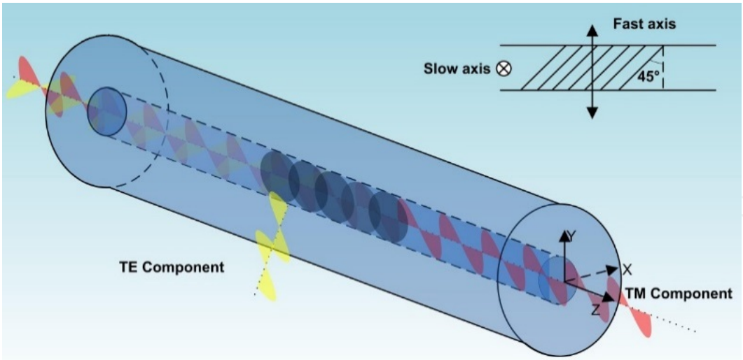
Figure 1. Schematic of 45°-TFG-based in-fiber polarizer.
