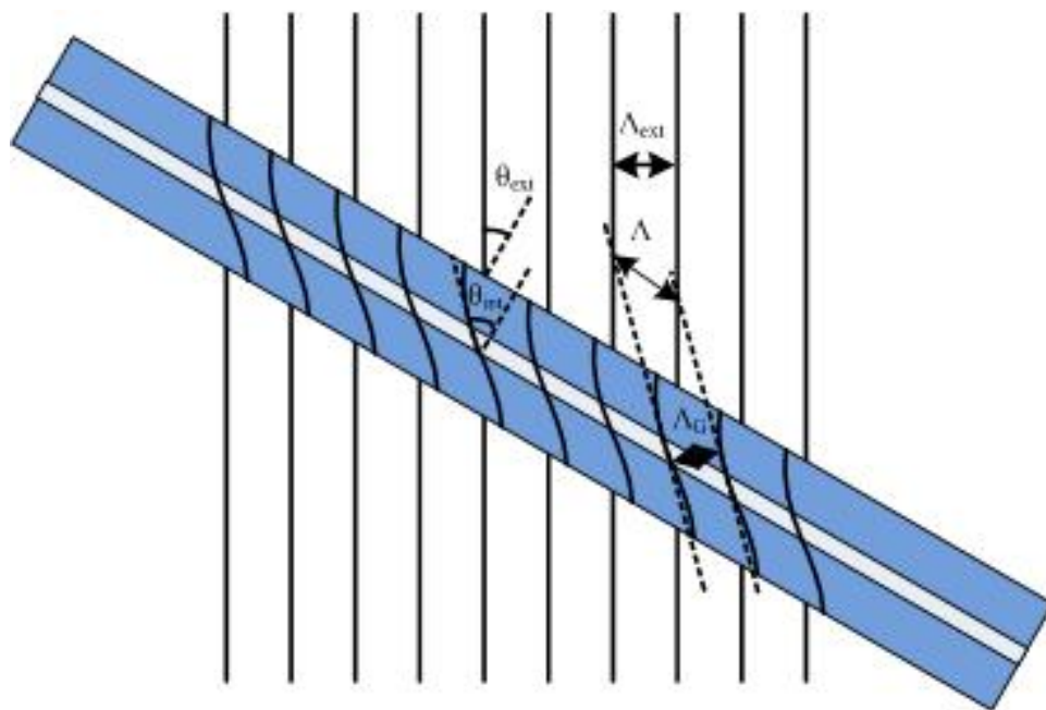
Figure 4. Illustration of fringes of a TFG outside and inside of the fiber with external angle \theta_{\text{ext}} and internal angle \theta_{\text{int}} .
