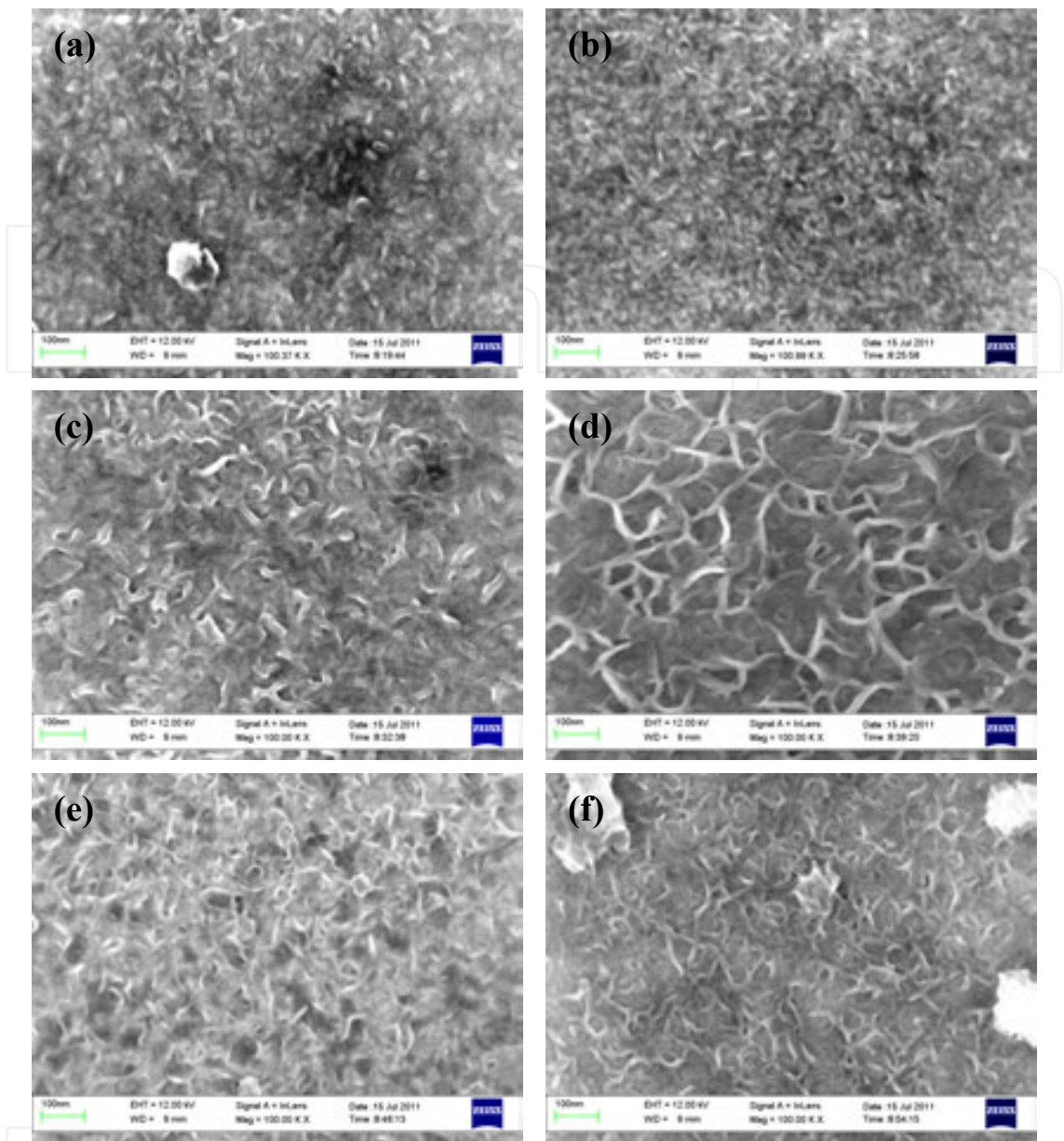
Figure 1. FE-SEM images showing the morphology of CoNi films electrodeposited with high magnetic fields of (a) 0 T, (b) 1 T, (c) 3 T, (d) 6 T, (e) 9 T, (f) 12 T.
