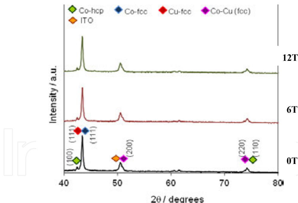
Figure 4. X-ray diffraction patterns of electrodeposited Co–Cu/Cu films with and without a superimposed magnetic field.
