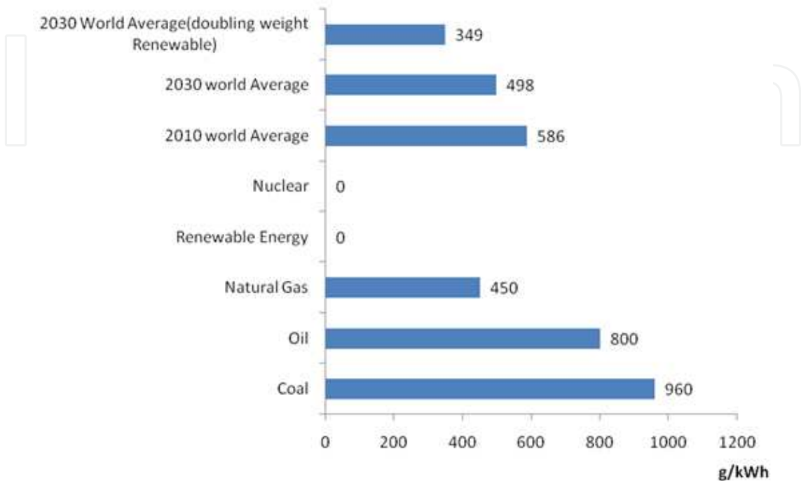
Figure 2. CO 2 emissions intensity
