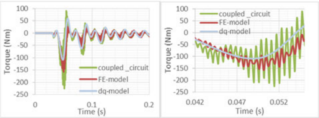
Figure 10: Electromagnetic torque (general pattern and detail 1) Figure 38. Electromagnetic torque (general pattern and detail 1)
