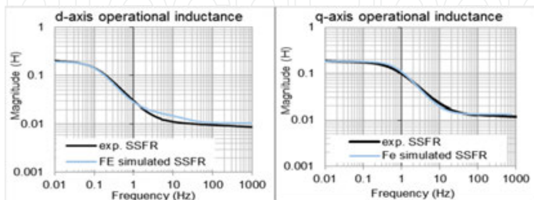
Figure 7: Comparison of experimental and simulated transfer functions
