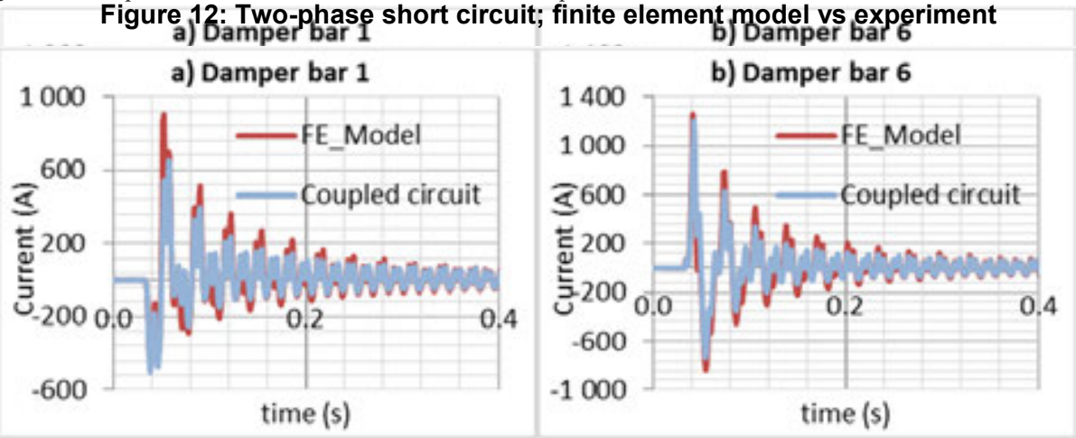
Figure 13: Two-phase short circuit; damper bar currents
