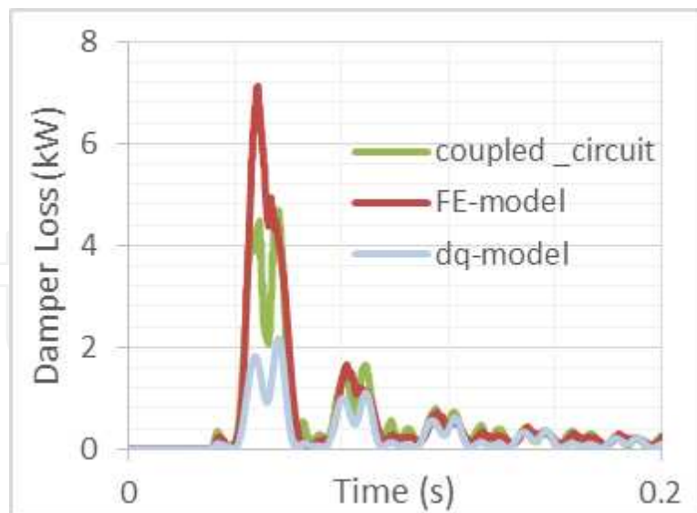
Figure 40. Copper losses of dumper circuit
